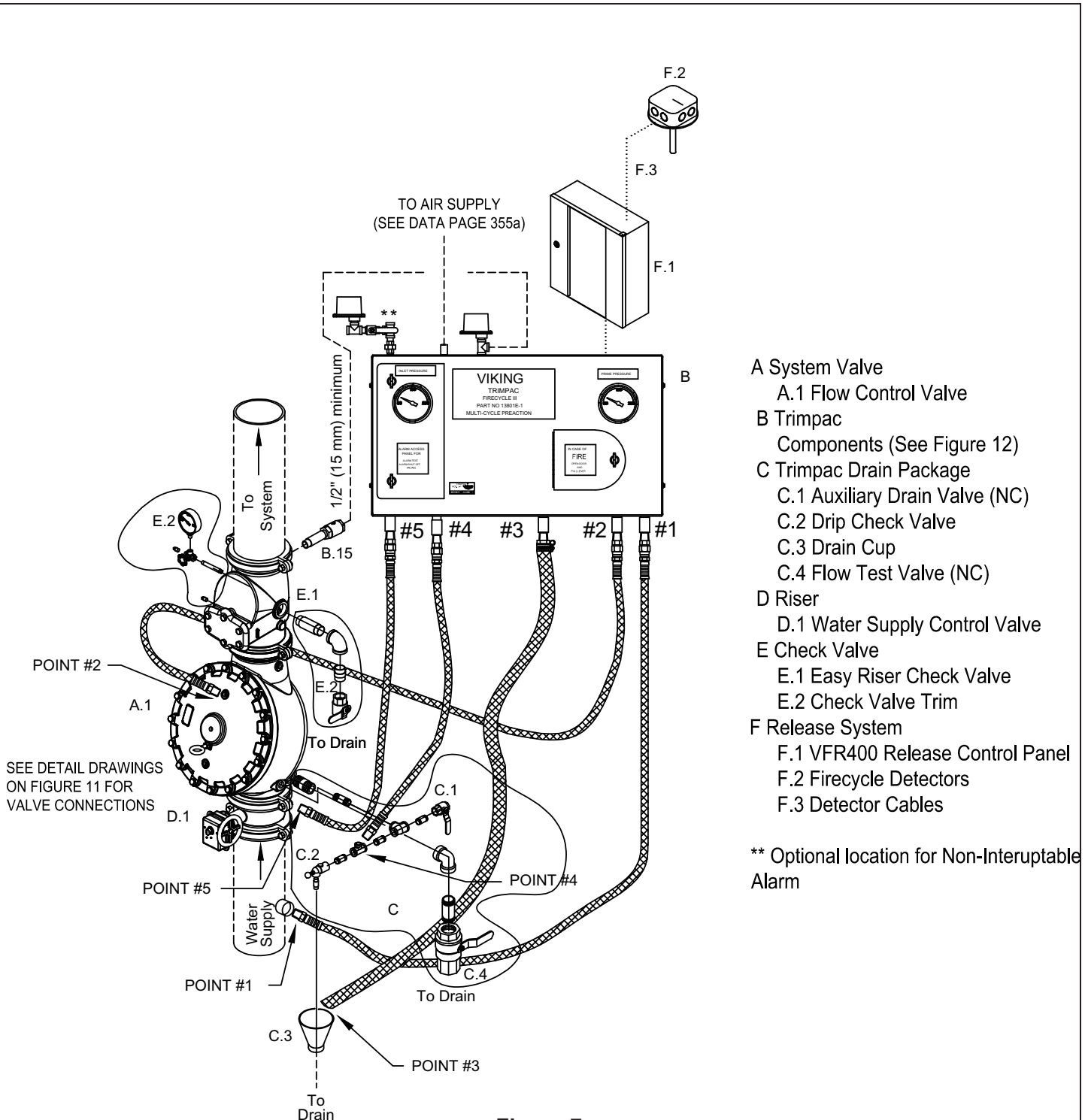
Figure 7 Firecycle® III Preaction System 8" Straight Through Vertical Valve
