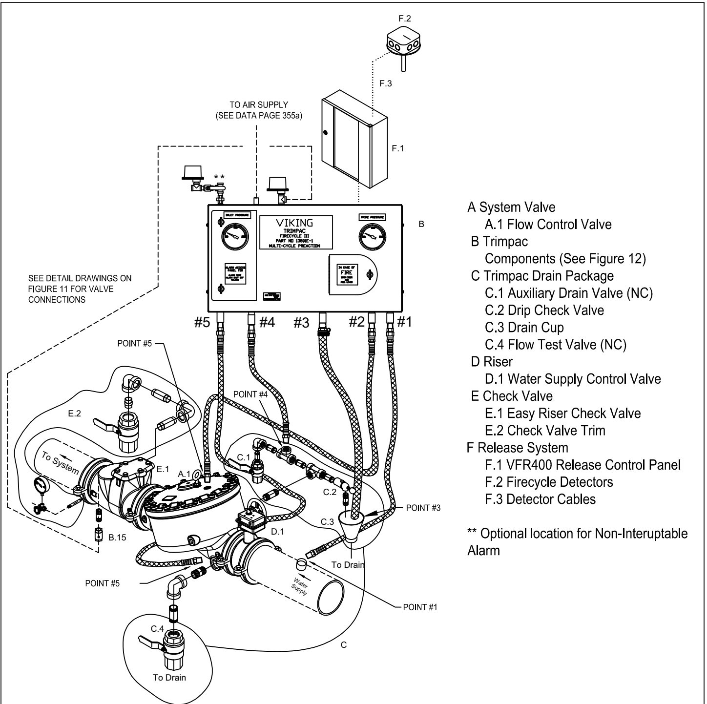
Figure 10 Firecycle® III Preaction System 8" Straight Through Horizontal Valve
