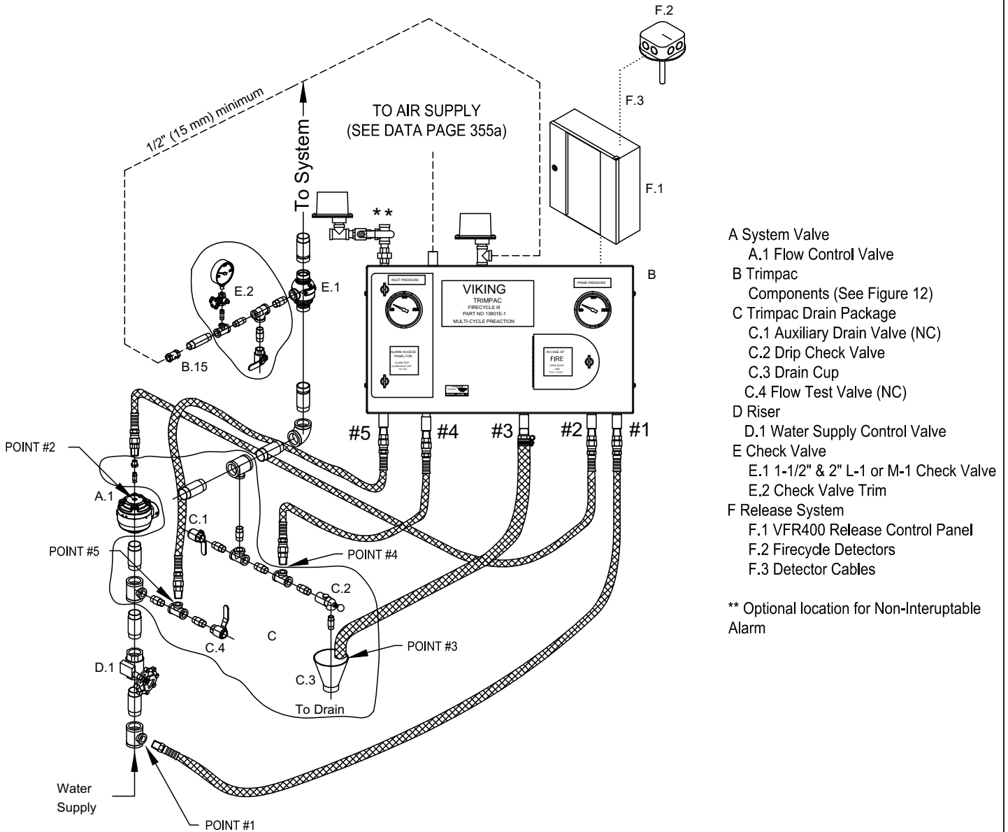
Figure 3 Firecycle® III Preaction System 1-1/2" Angle Style Valve
