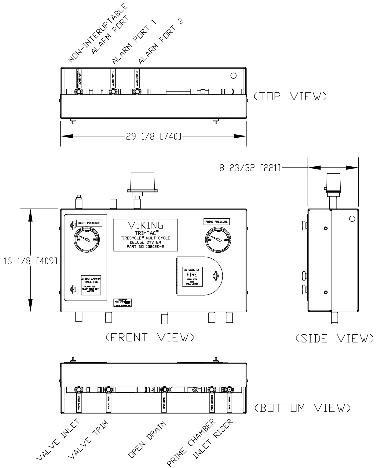
Figure 2 - Trimpac® Model E-2 Dimensions
