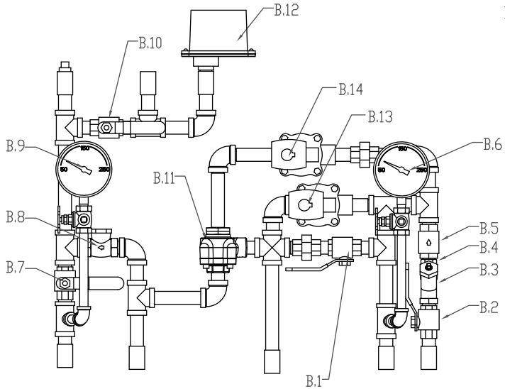
Figure 12 - Trimpac® Components (Items B.1 - B.14)
