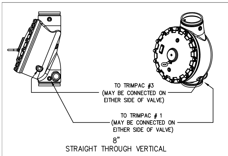
Figure 11 - Valve Connections
