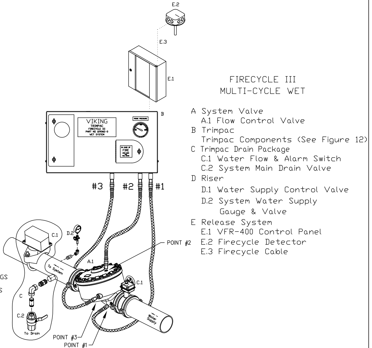
Figure 8 Firecycle® III Wet System 2-1/2" - 6" Straight Through Horizontal Valve
