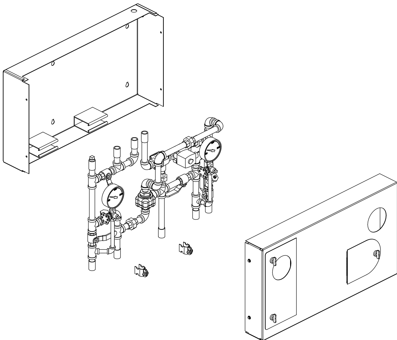
Figure 1 - Isometric View
