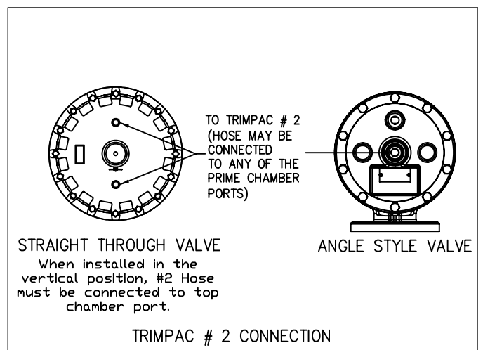
Figure 11 - Valve Connections
