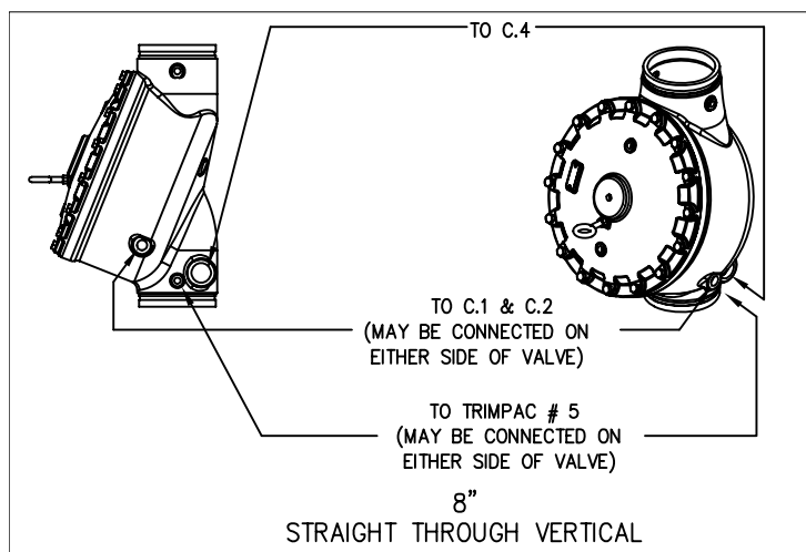
Figure 11 - Valve Connections
