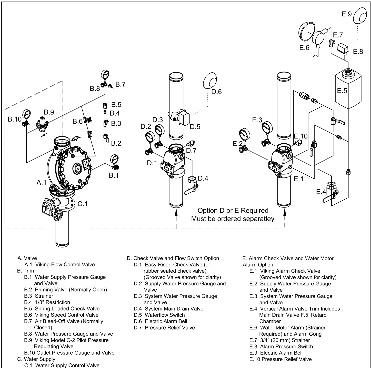
Figure 1 - Vertical Installation System Components
