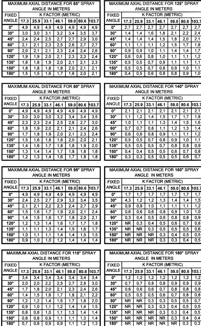
Figure 6b: Maximum Axial Distance Between Nozzle Tip and Plane of Protection for Exposure Protection (m)
