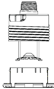
Cover Plate Assembly (Pendent Cover 13504 shown)
