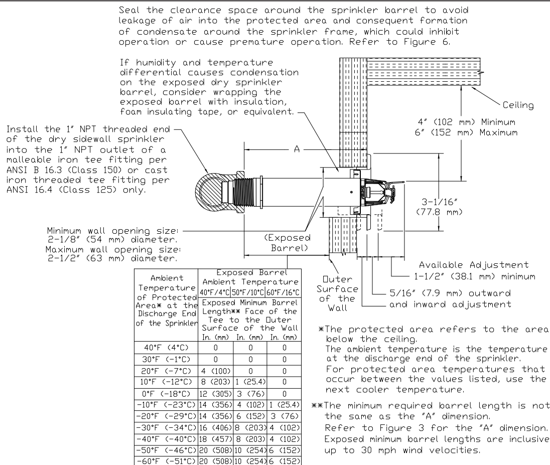
Figure 5: Dry Horizontal Sidewall Sprinkler Required Minimum Barrel Length Based on Ambient Temperature in the Protected Area
