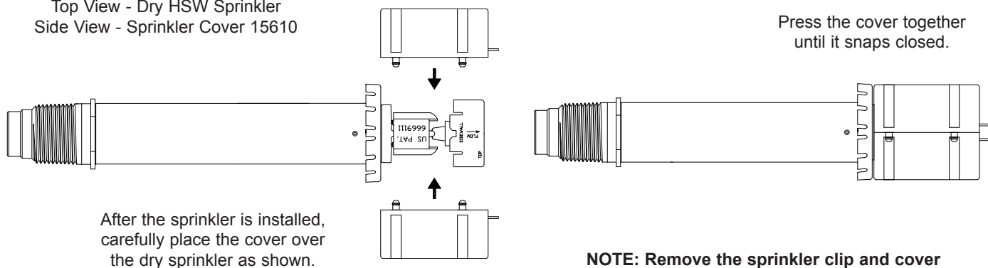
Figure 4: Dry Horizontal Sidewall Sprinkler Cover Part Number 15610
