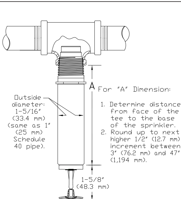
Figure 4: Adjustable Standard Dry Pendent Sprinkler
