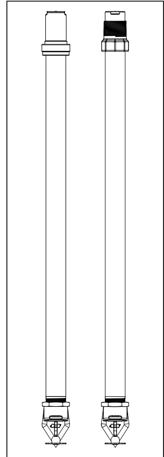
ESFR Sprinkler VK502 (Grooved and Threaded)
