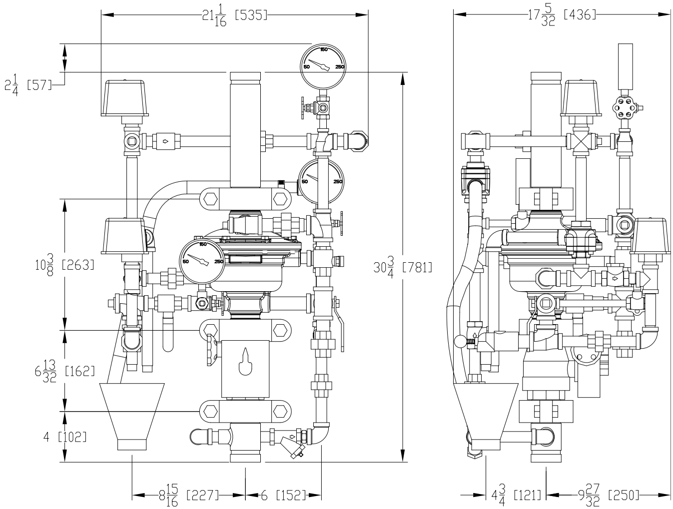
Figure 10 - Installation Dimensions
