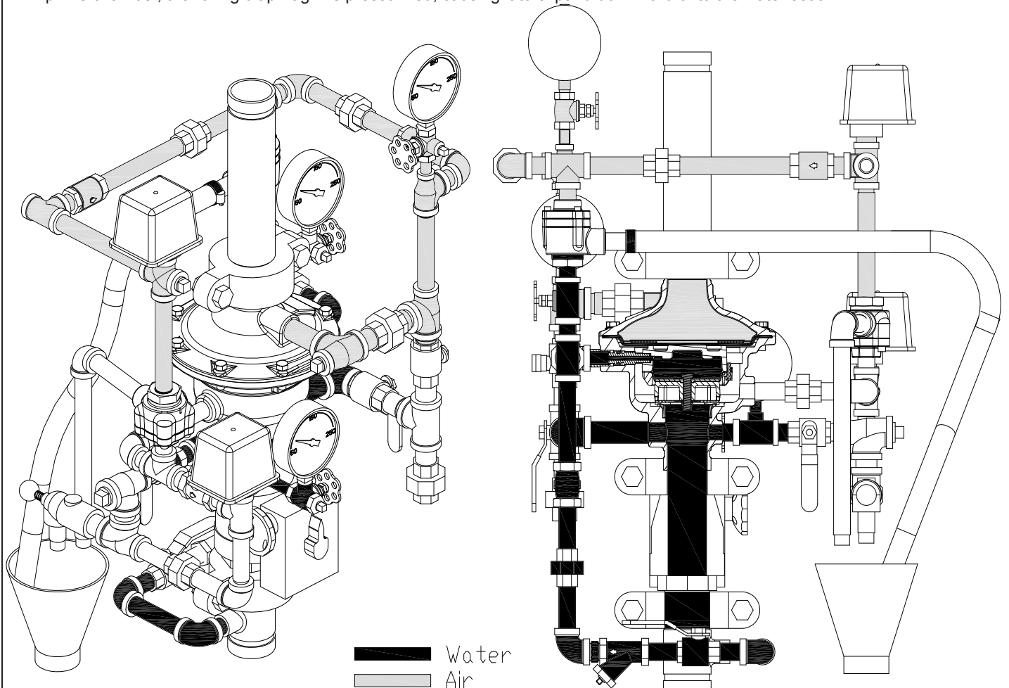
Figure 6 - Set Position
