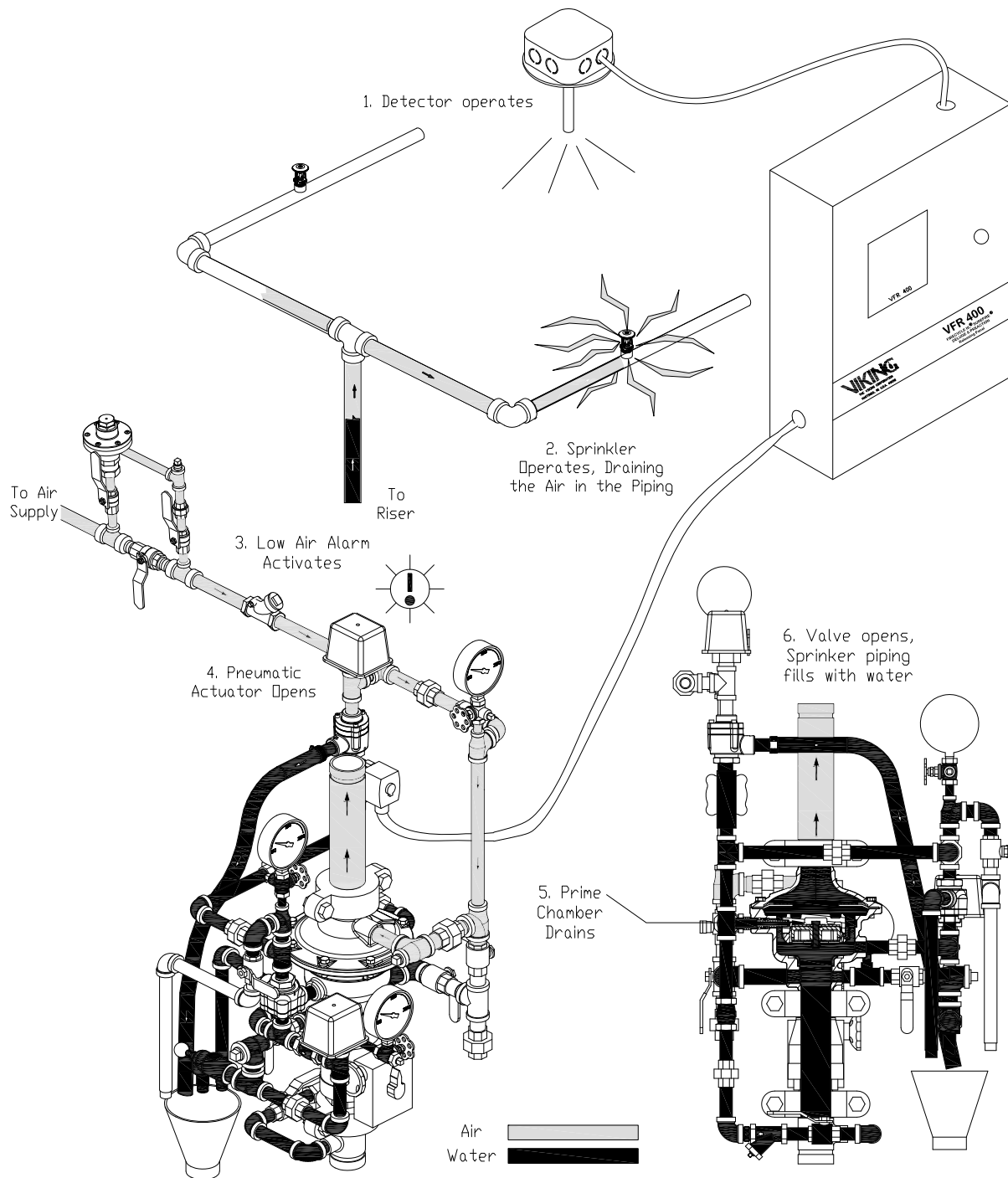
Figure 7 - Fire Condition
