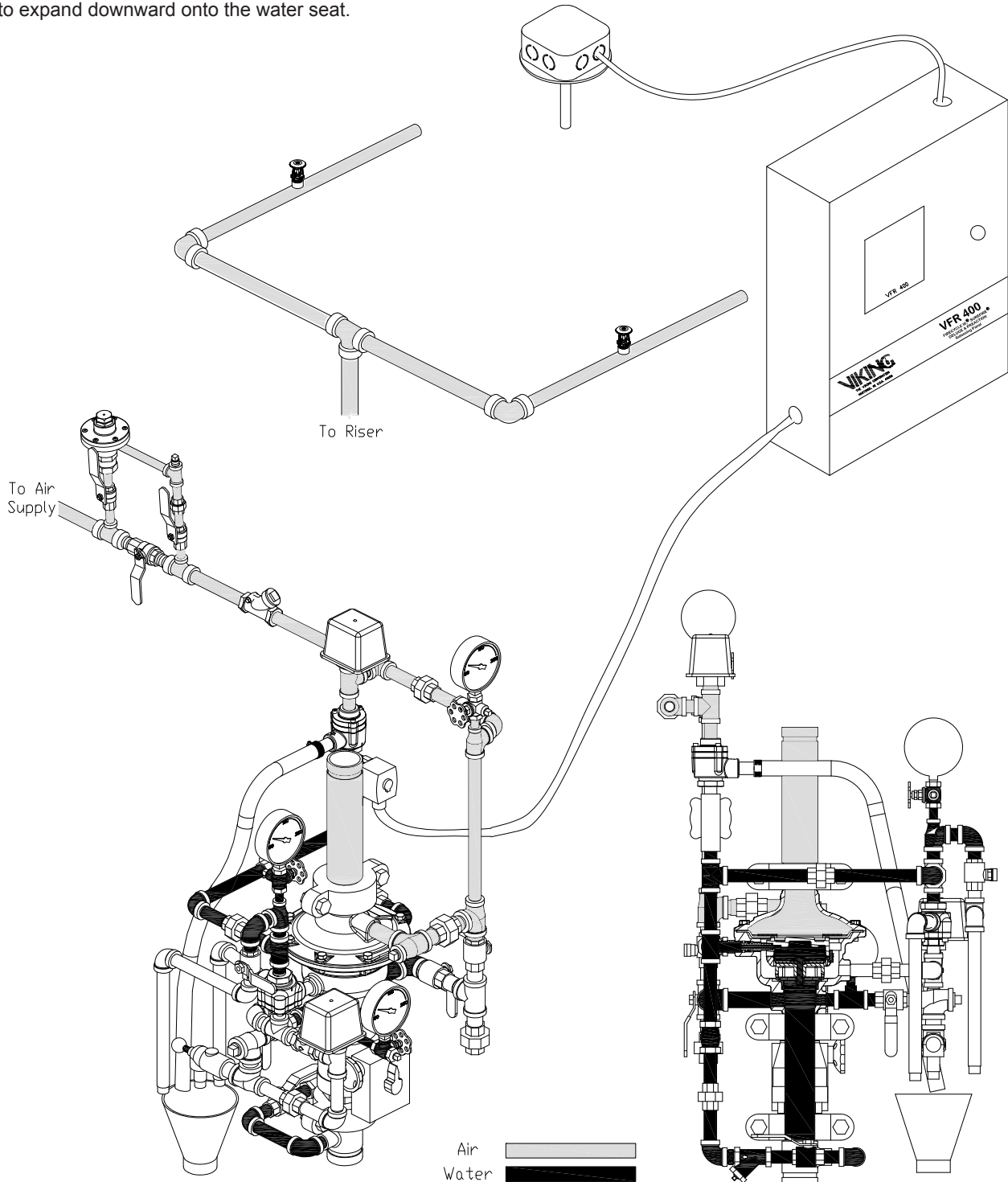
Figure 6 - Set Position
