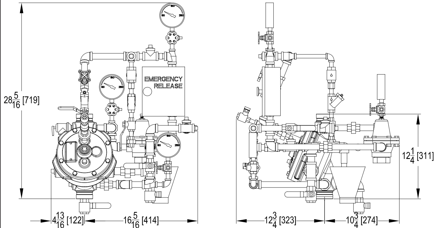
Figure 2 - Installation Dimensions
