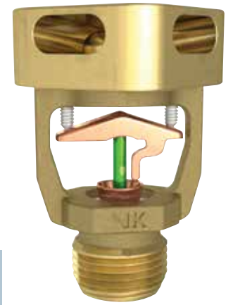
NEW V-HIP VK660 Attic Hip 5.6 K-factor
