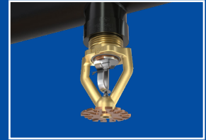
A fully installed ESFR sprinkler
