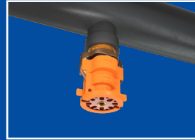
Viking ESFR sprinkler featuring the Torque-Assist Cap hand-tightened into the welded outlet
