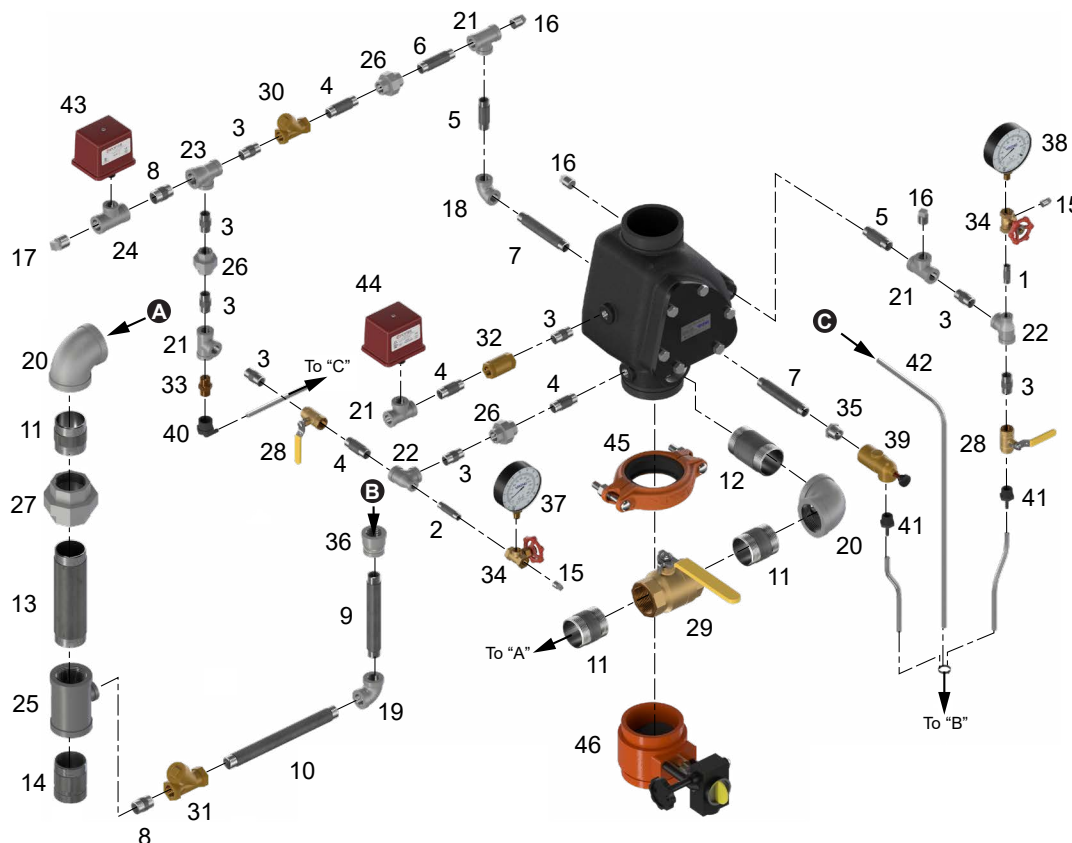
Figure 14: Trim Diagram - PTR (4")
