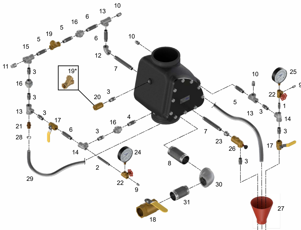
Figure 17: Trim Diagram - Standard Trim (6'')
