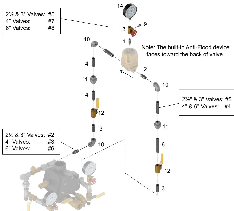
Figure 18: Accelerator (Model D-2) Trim Diagram - 2 1/2" Shown
