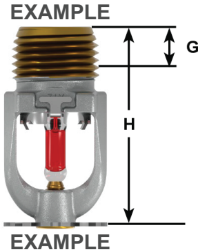
Figure – 2: Dimensions
