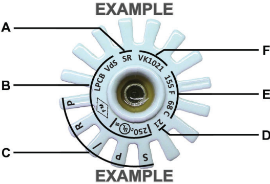
Figure – 1: Markings
