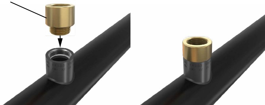
Figure 3: Pipe Adapter Bushing Installation
