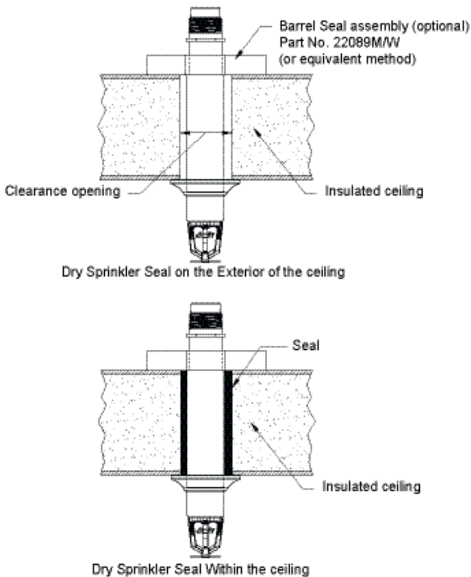
Figure 6: Dry Sprinkler Seal (Adjustable Standard Dry Pendent Sprinkler is Shown)
