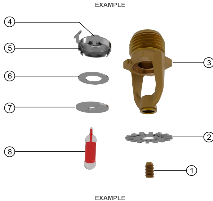
Figure – 3: Sprinkler Components
