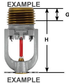
Figure – 2: Dimensions
