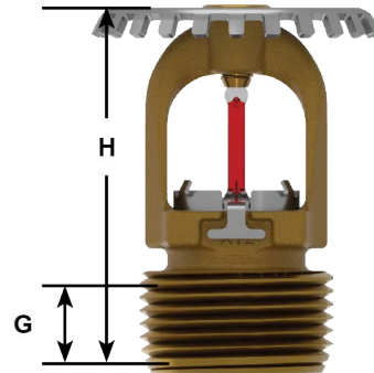
Figure – 2: Dimensions
