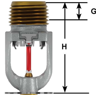
Figure – 2: Dimensions
