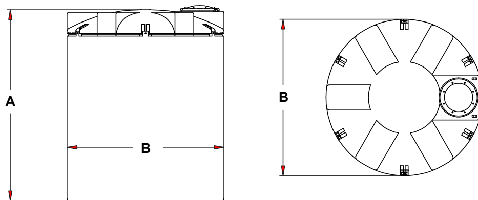
Figure 6.2.1 - SAFE Tank Dimensions
