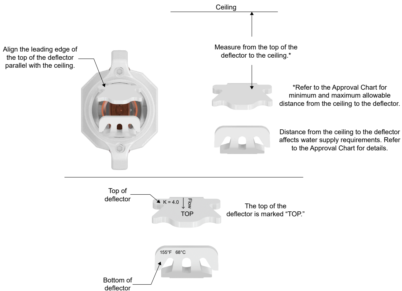
Figure 3: Correct Orientation of the Deflector
