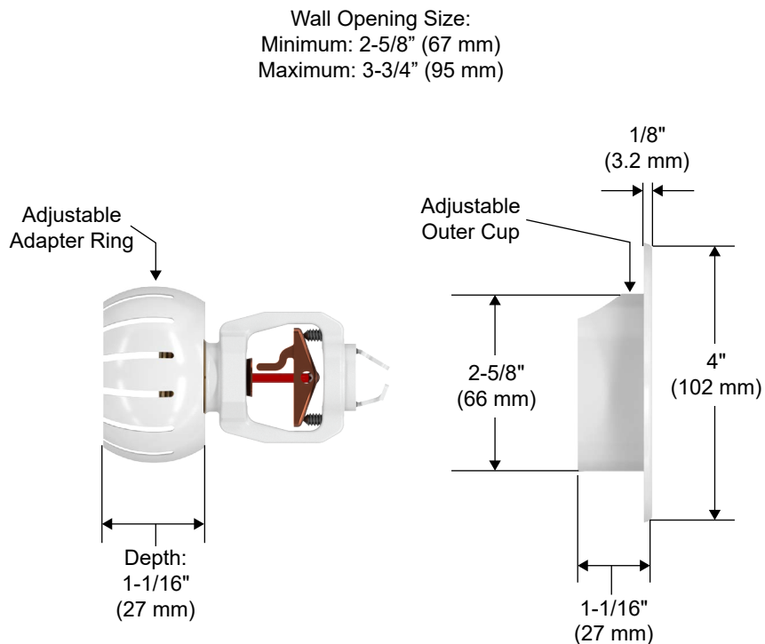
Figure 6: Sprinkler VK4860 Dimensions with the Model G-1 Escutcheon
