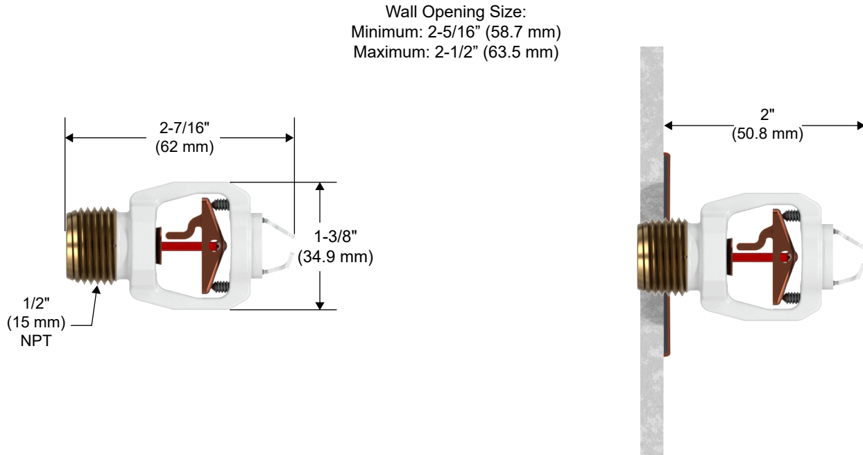
Figure 4: Sprinkler VK4860 Dimensions with a Standard Escutcheon
