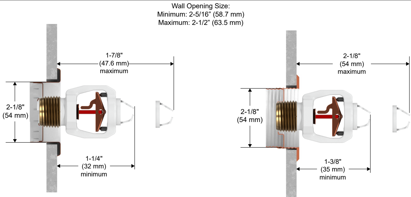
Figure 5: Sprinkler VK4860 Dimensions with the Model E-1 and E-2 Recessed Escutcheons
