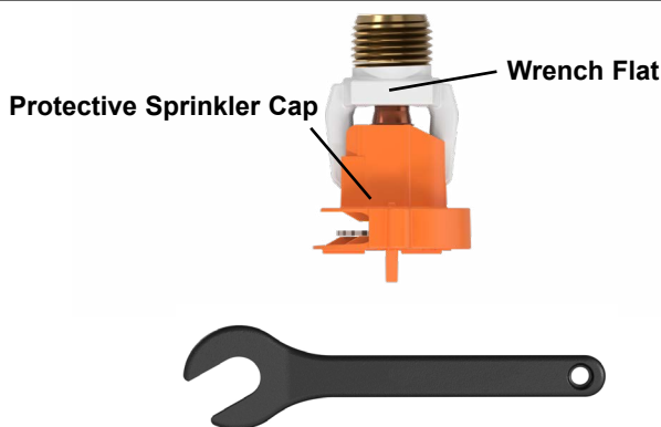
Figure 1: Sprinkler with Torque Assist Cap and Sprinkler Wrench 21475M/B
