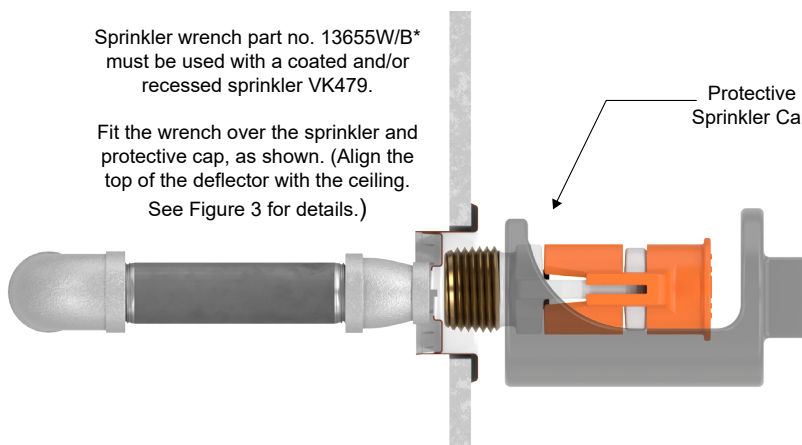
Figure 2: Recessed Sprinkler VK479 with Torque Assist Cap
