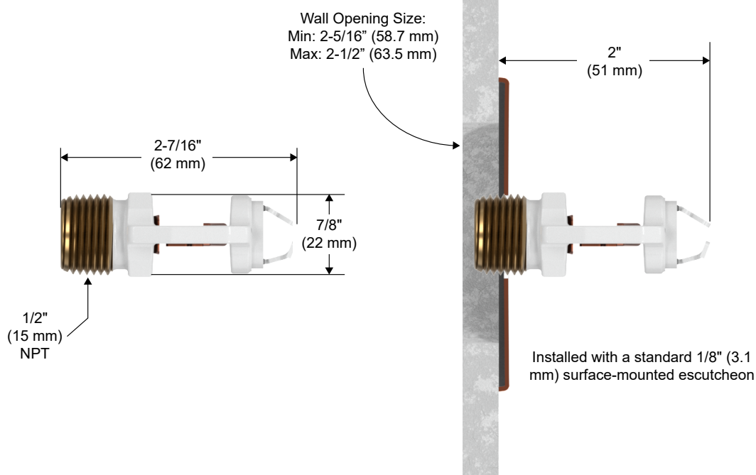
Figure 4: Sprinkler VK479 Dimensions with a Standard Escutcheon
