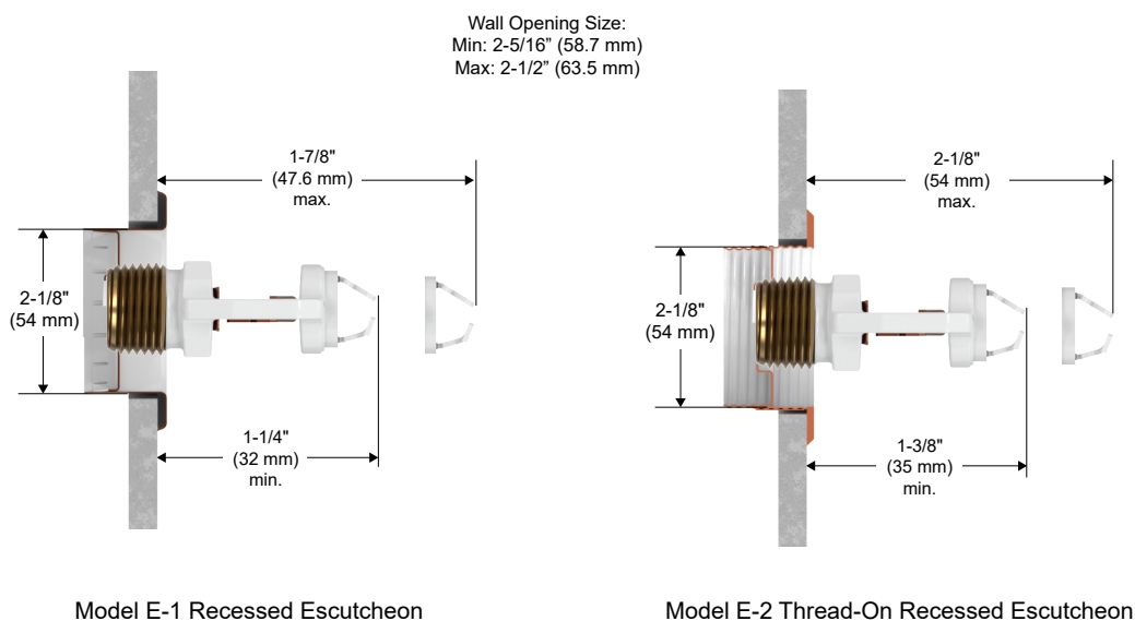
Figure 5: Sprinkler VK479 Dimensions with the Model E-1 and E-2 Recessed Escutcheons
