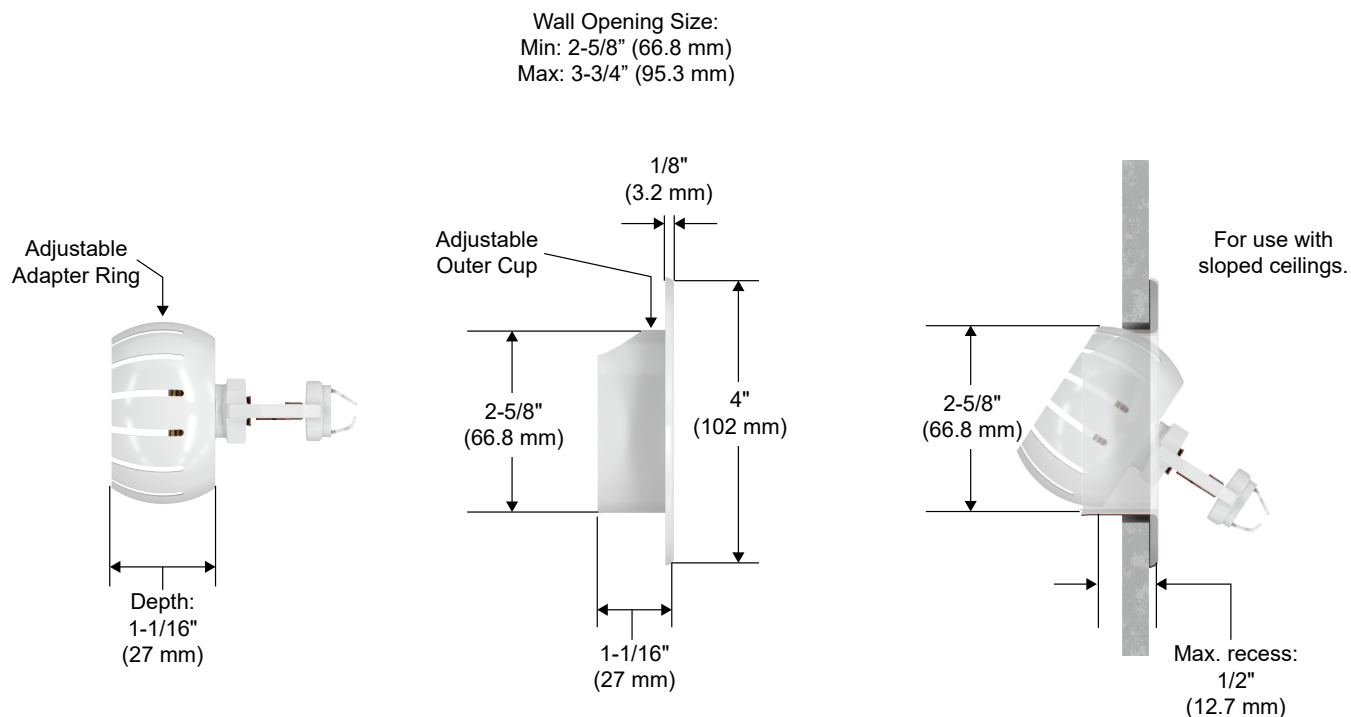
Figure 6: Sprinkler VK479 Dimensions with the Model G-1 Escutcheon
