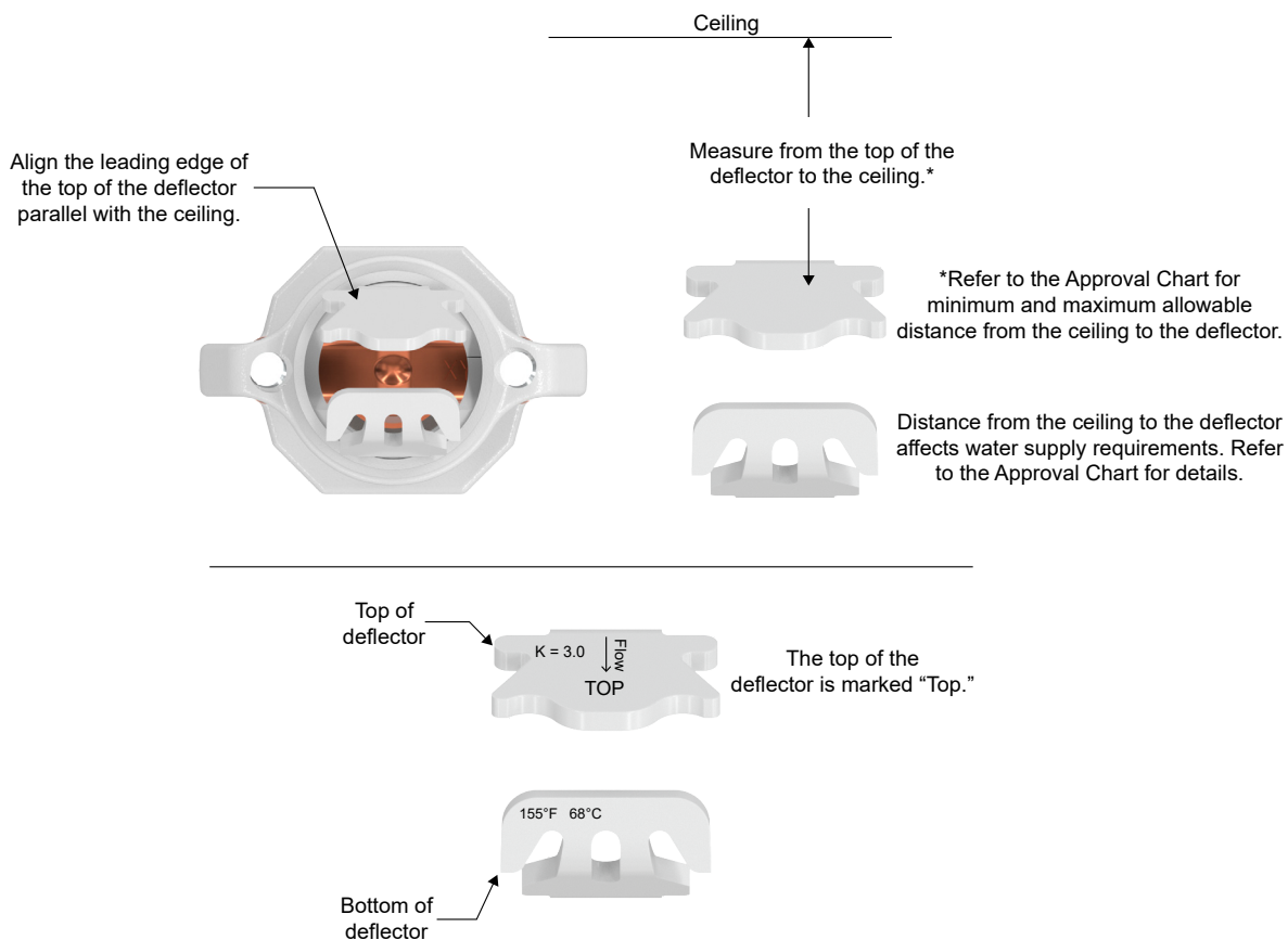
Figure 3: Correct Orientation of the Deflector
