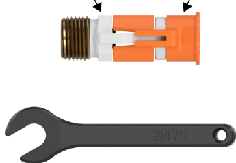
Figure 1: Sprinkler with Torque Assist Cap
