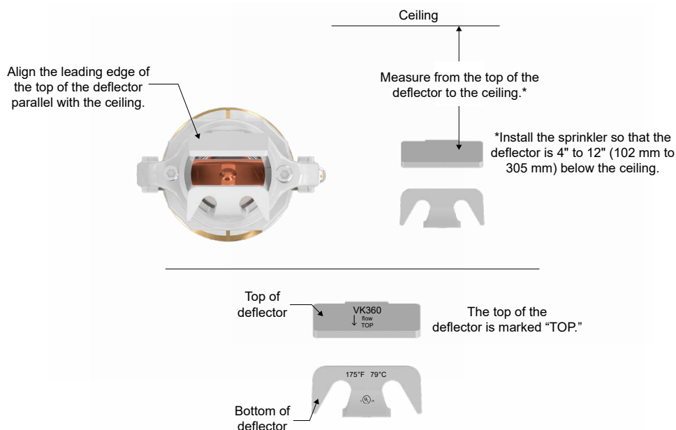
Figure 3: Correct Deflector Orientation
