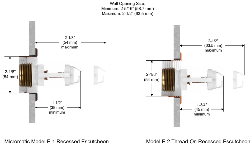
Figure 5: Sidewall Sprinkler VK360 Dimensions with the Model E-1 and E-2 Recessed Escutcheons
