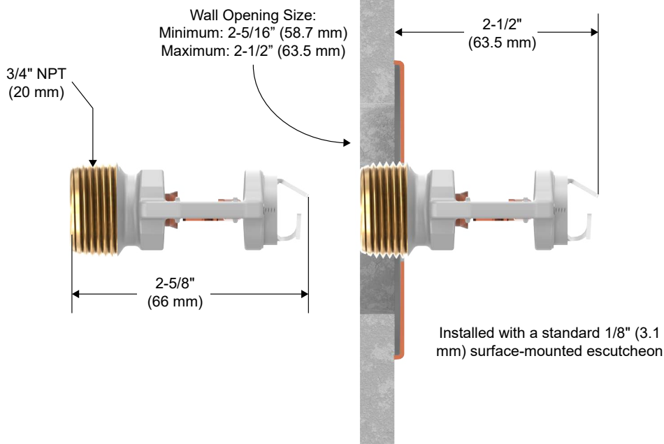
Figure 4: Sidewall Sprinkler VK360 Dimensions with a Standard Escutcheon
