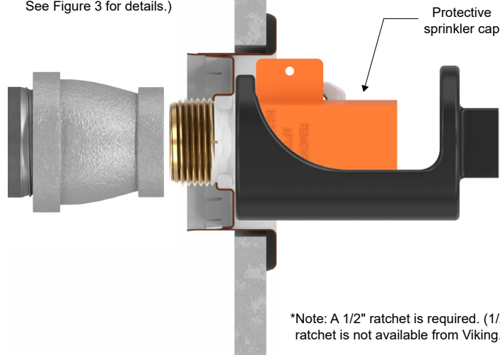
Figure 2: Installation of Coated and/or Recessed Sprinkler VK360
