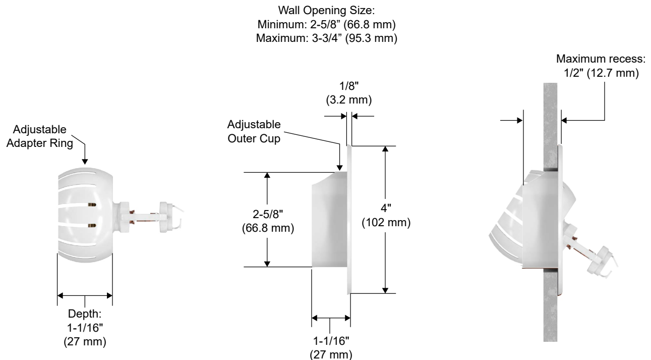
Figure 6: Sprinkler VK360 Dimensions with the Model G-1 Escutcheon
