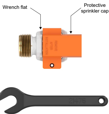
Figure 1: Standard Sprinkler Wrench 21475M/B
