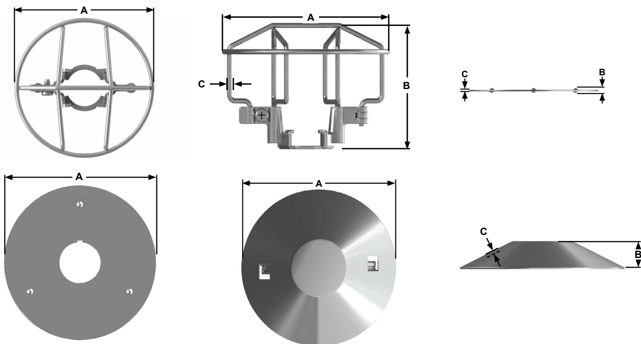
Figure 1: Dimensions
