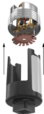
Figure 6: Sprinkler Installation
