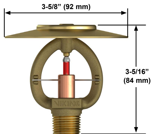
Figure 2: Sprinkler VK540 Dimensions
