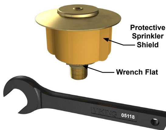
Figure 1: Sprinkler Wrench 05118CW/B
