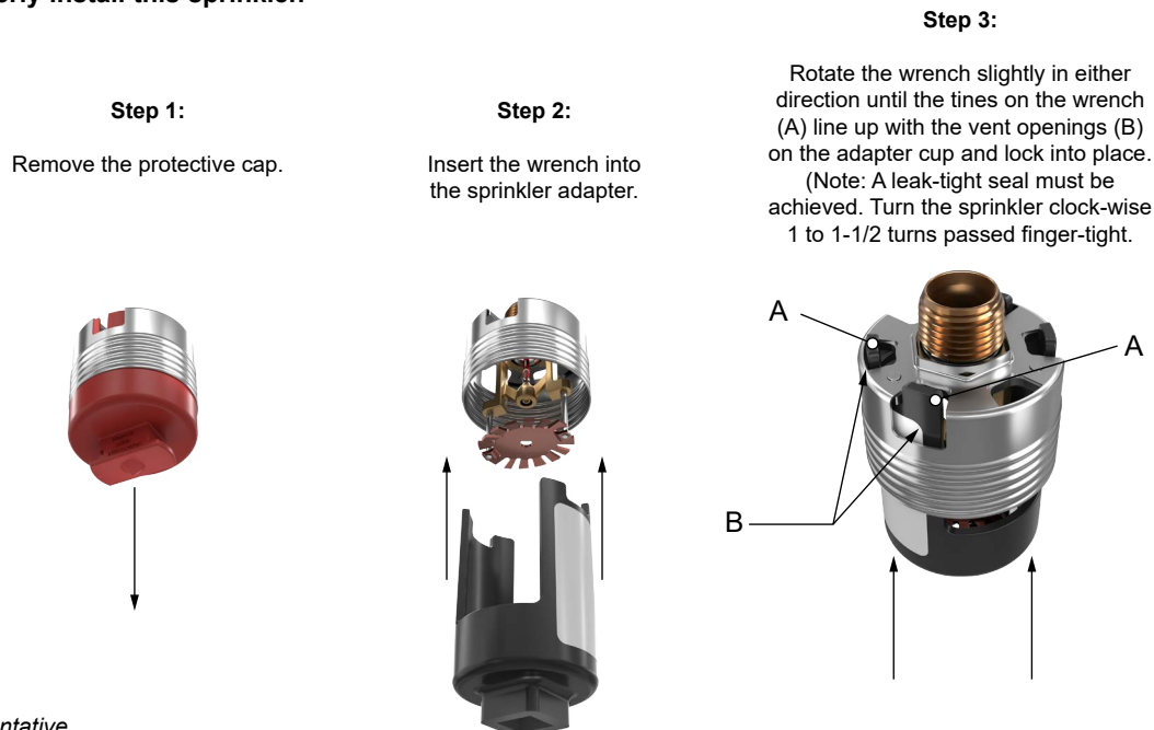
Figure 6: Using the Sprinkler Wrench
