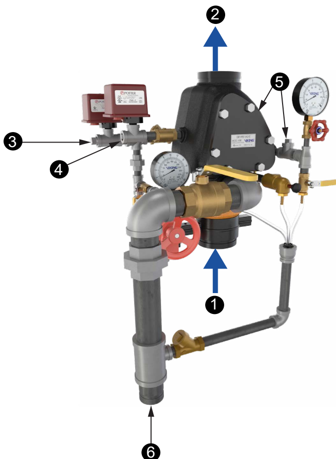
Figure 6: System Connection Points (4" PTR Shown)
