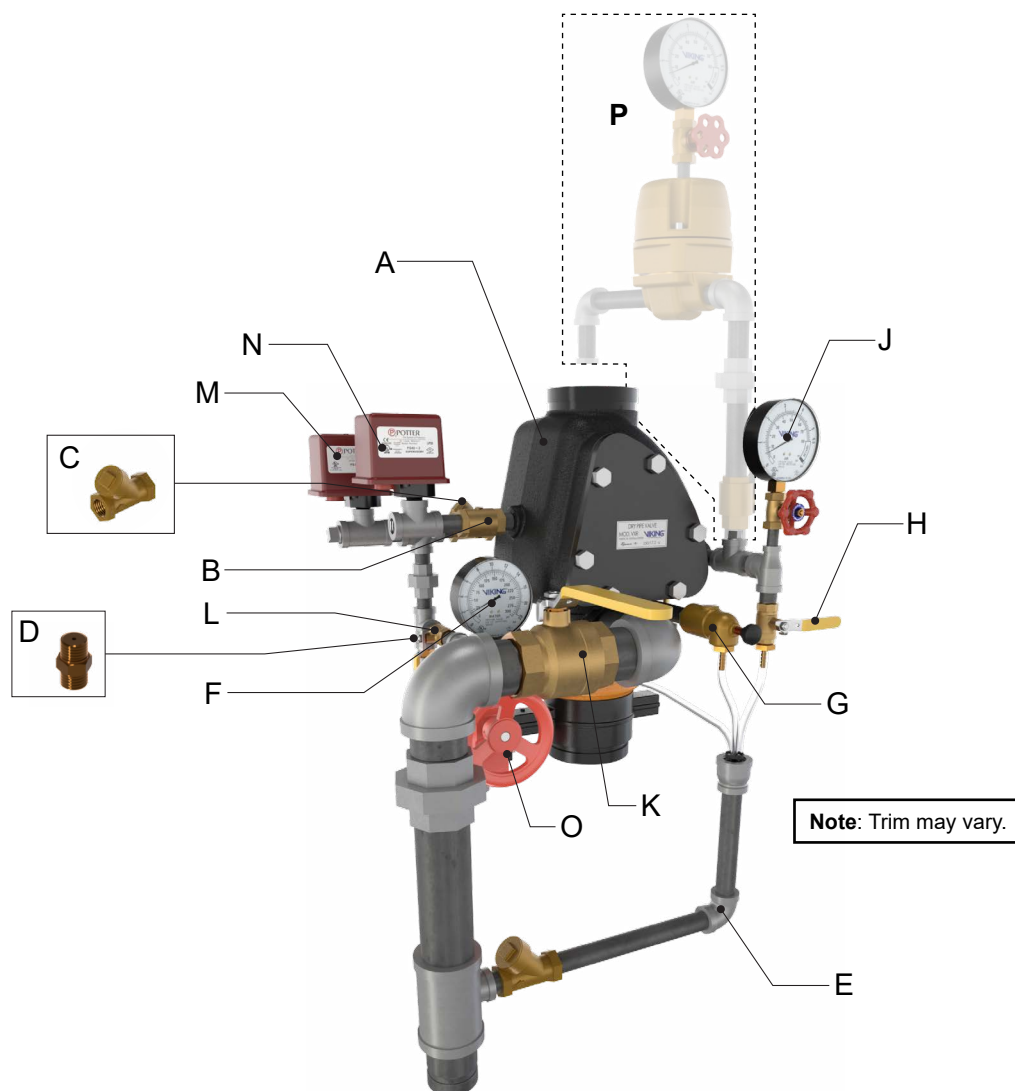
Figure 4: System Components (4" PTR Shown)
