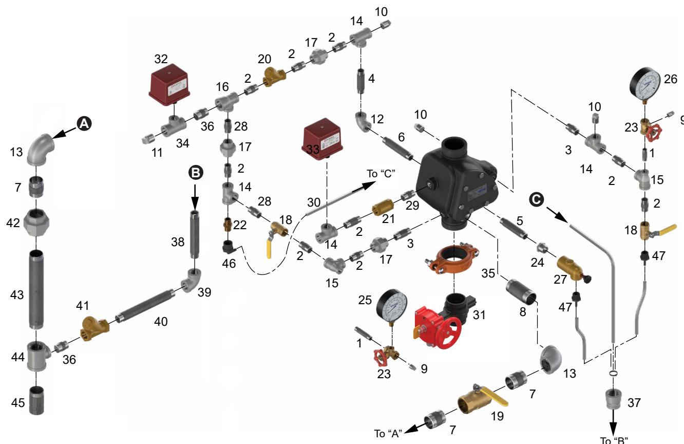
Figure 10: Trim Diagram - PTR (2½")
