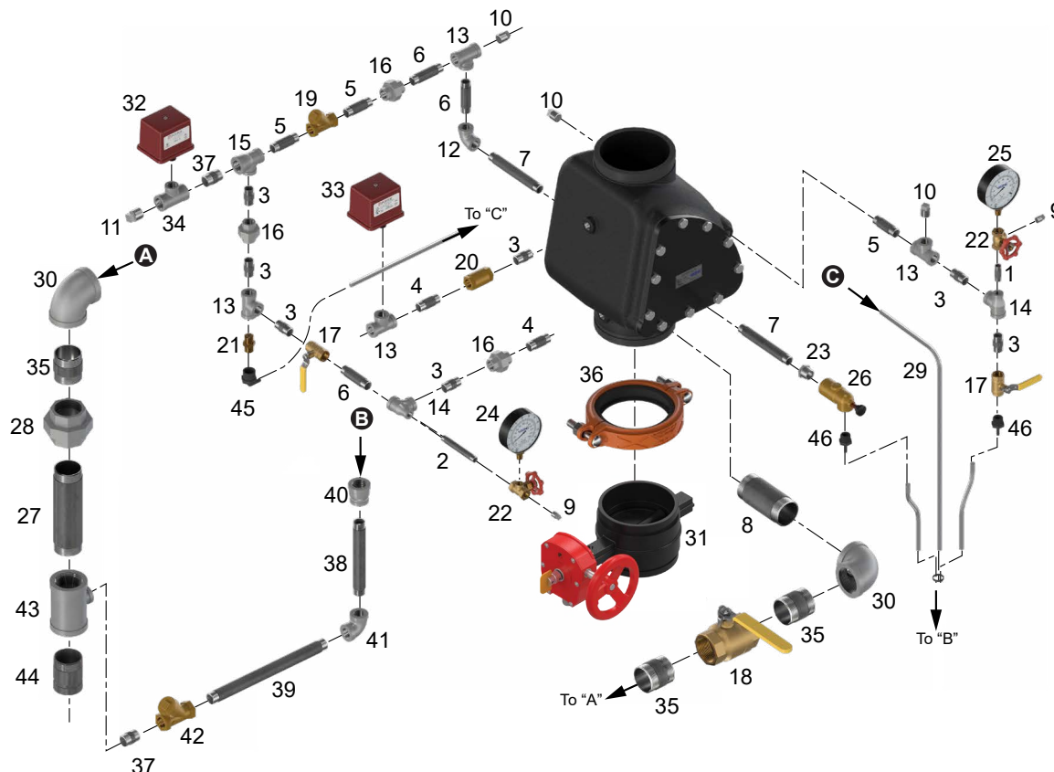
Figure 16: Trim Diagram - PTR (6")
