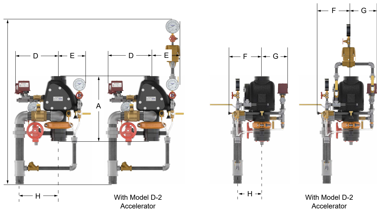
Figure 9: System Dimensions for Pre-Trimmer Risers (PTR) (4" Pre-Trimmed Risers Shown)
