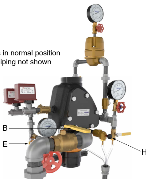
Figure 7: Water Flow and Alarm Test
