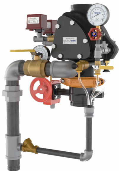
Figure 1: Pre-Trimmed Riser (PTR) Configuration
