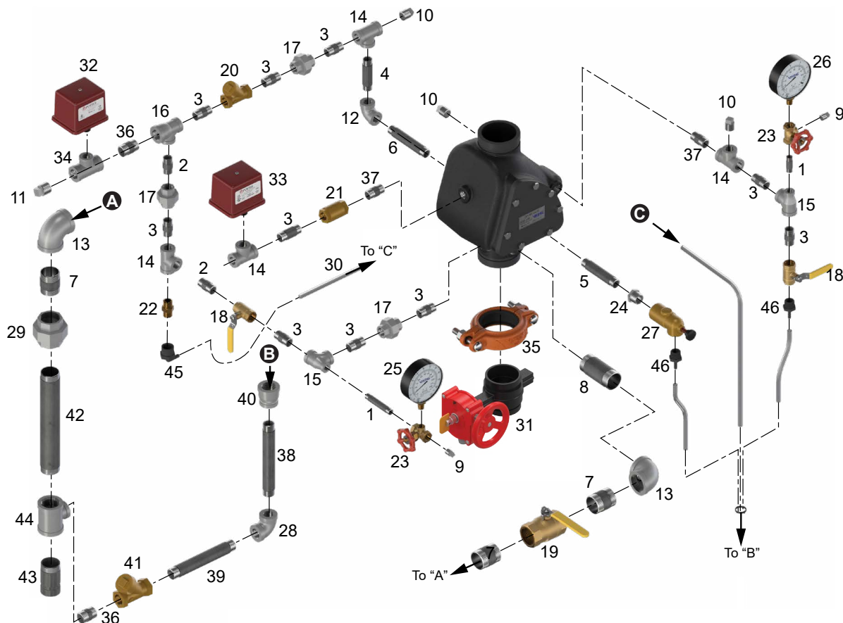
Figure 12: Trim Diagram - PTR (3")
