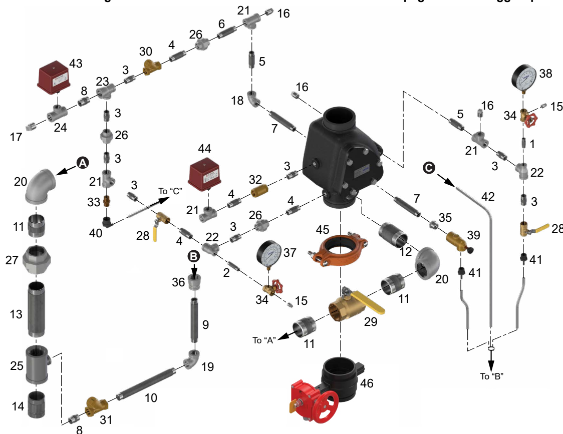
Figure 14: Trim Diagram - PTR (4")
