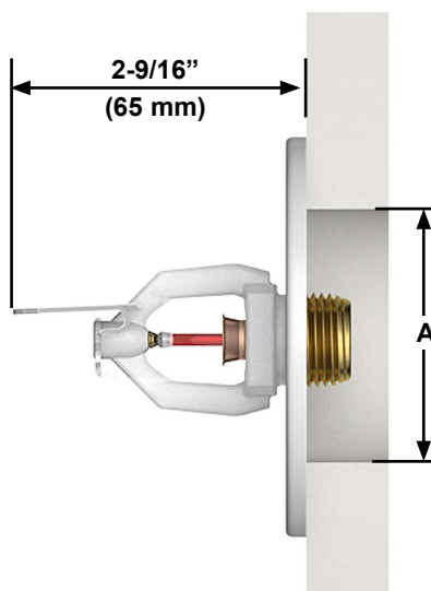
Figure 3: Sprinkler VK484 Dimensions with a Standard Surface-Mount Escutcheon
