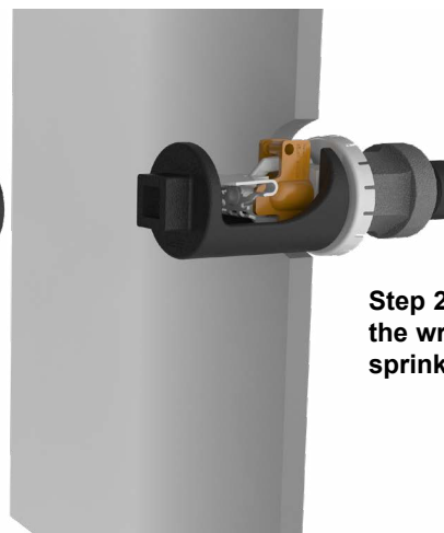
Figure 2: Wrench 13655W/B for Recessed Sprinkler VK484
