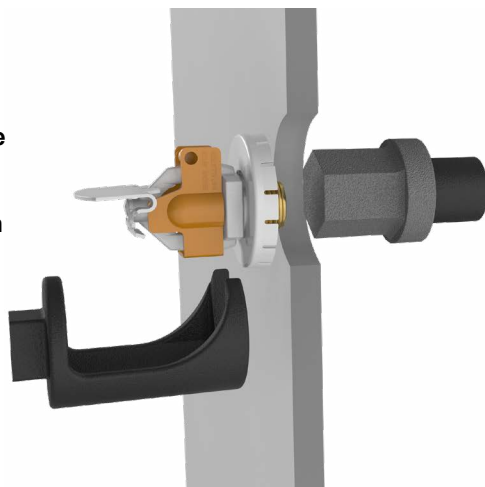
Figure 2: Wrench 13655W/B for Recessed Sprinkler VK484
