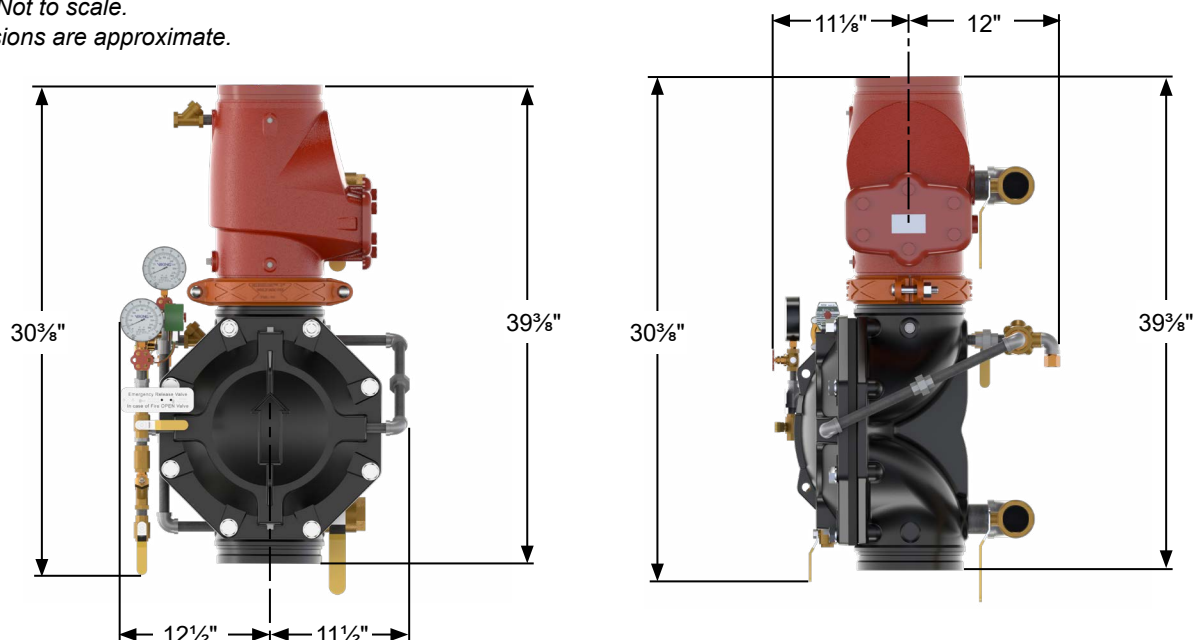
Figure 21: Dimensions - 8" LoosePre-trimmed
