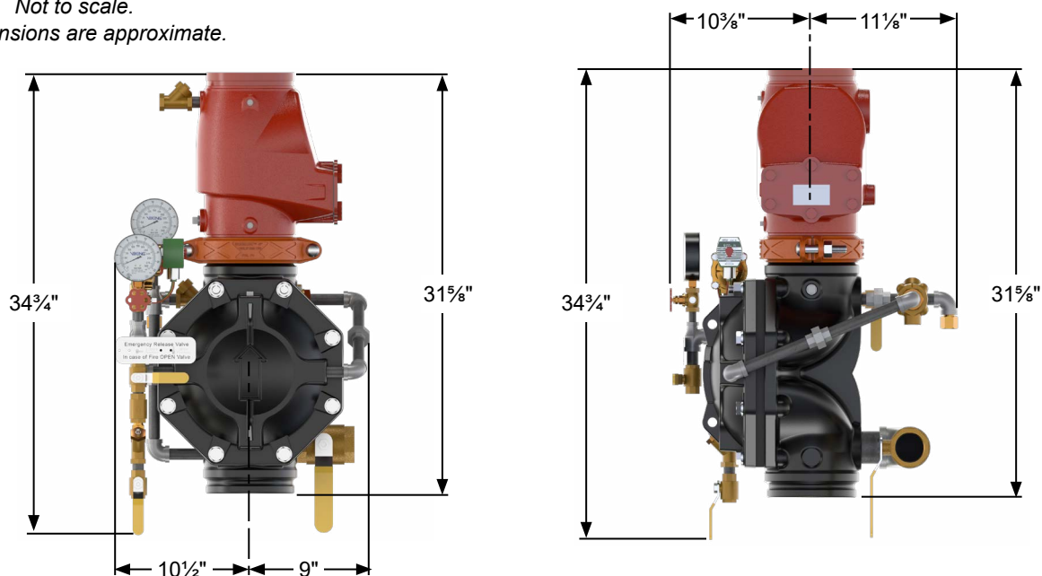
Figure 19: Dimensions - 6" LoosePre-trimmed
