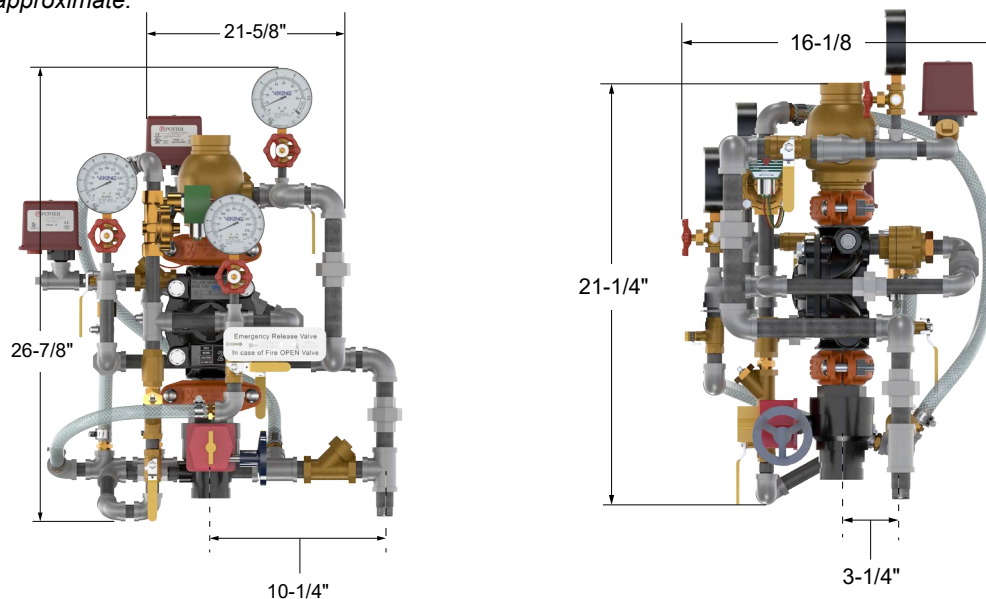
Figure 10: Dimensions - 2" Pre-trimmed Riser
