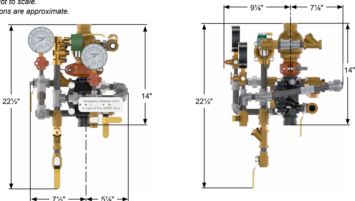
Figure 9: Dimensions - 1.5" Loose/Pre-trimmed
