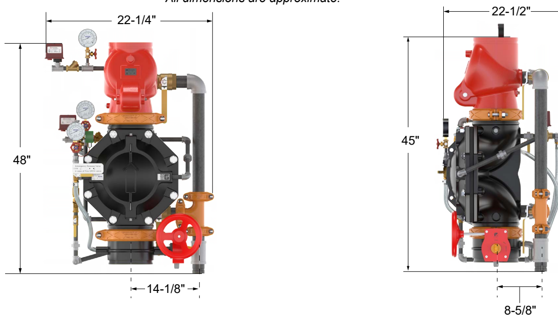
Figure 20: Dimensions - 8" Pre-trimmed Riser
