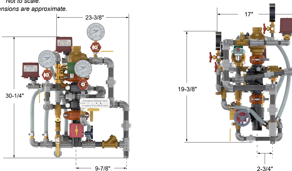
Figure 8: Dimensions - 1.5" Pre-trimmed Riser
