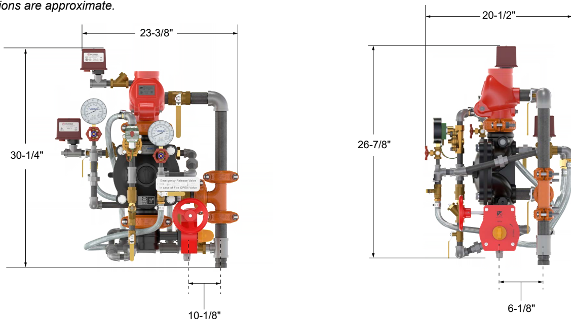
Figure 14: Dimensions - 3" Pre-trimmed Riser
