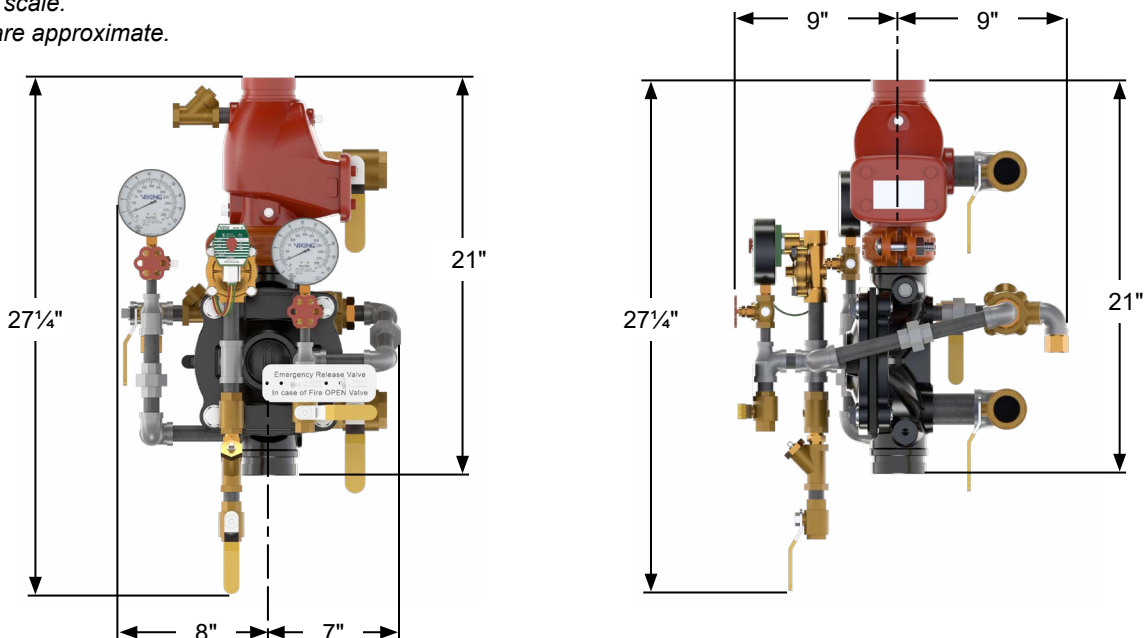
Figure 13: Dimensions - 2.5" Loose/Pre-trimmed
