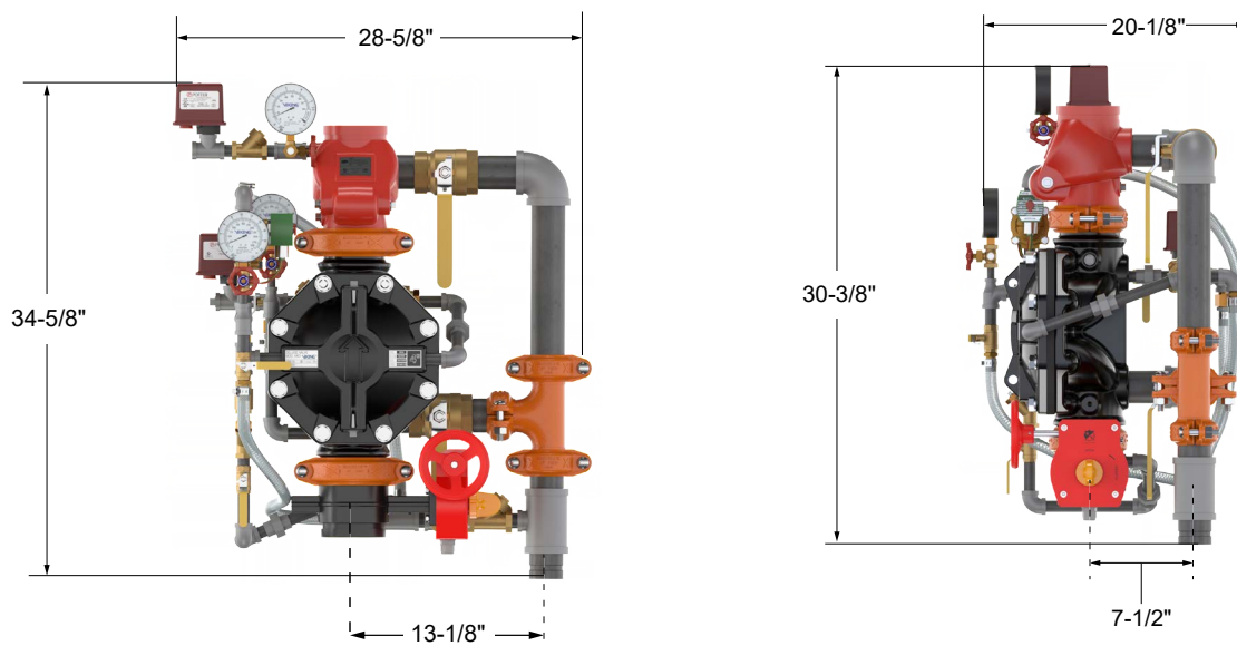
Figure 16: Dimensions - 4" Pre-trimmed Riser
