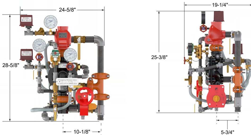
Figure 12: Dimensions - 2.5" Pre-trimmed Riser
