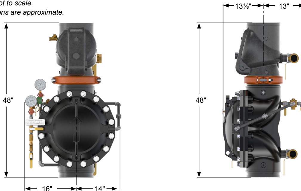
Figure 22: Dimensions - 10" Loose/Pre-trimmed
