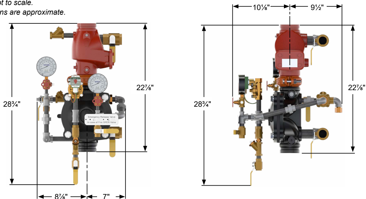
Figure 15: Dimensions - 3" Loose/Pre-trimmed
