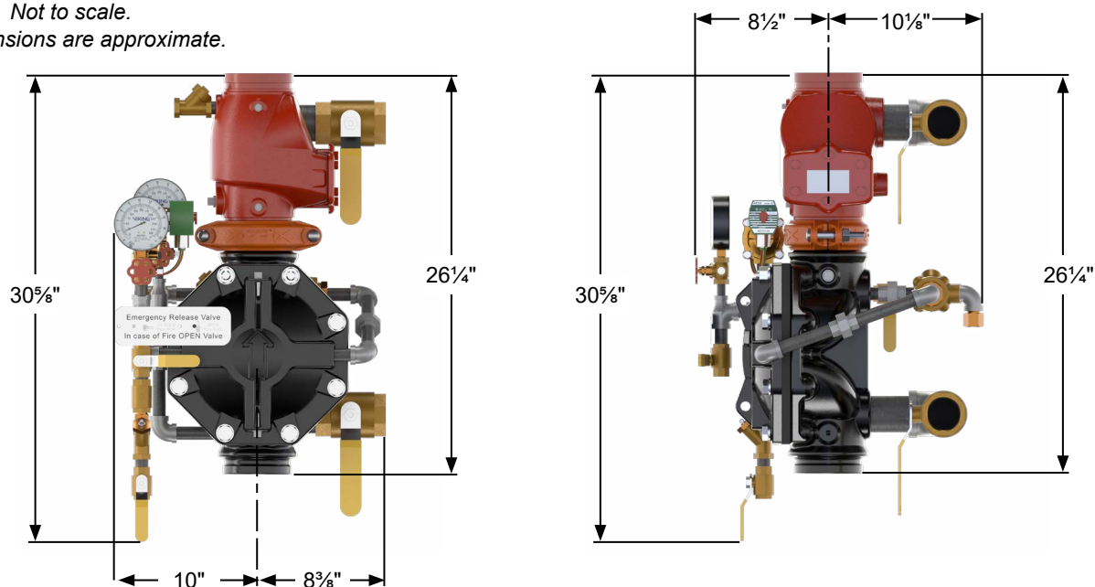
Figure 17: Dimensions - 4" LoosePre-trimmed
