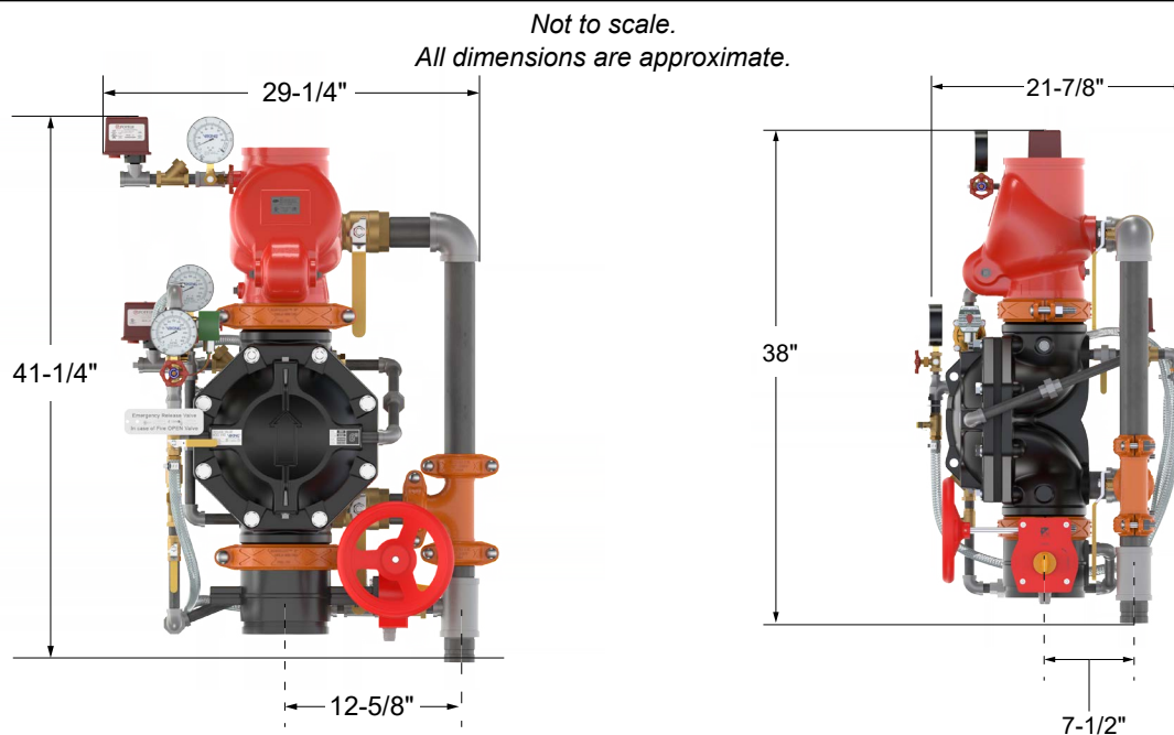
Figure 18: Dimensions - 6" Pre-trimmed Riser
