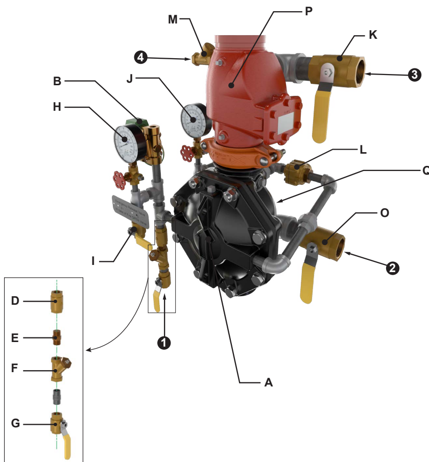
Figure 4: System Components (4\"
