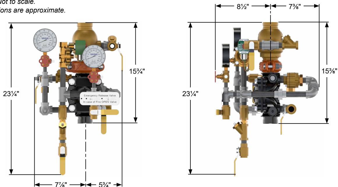
Figure 11: Dimensions - 2" Loose/Pre-trimmed
