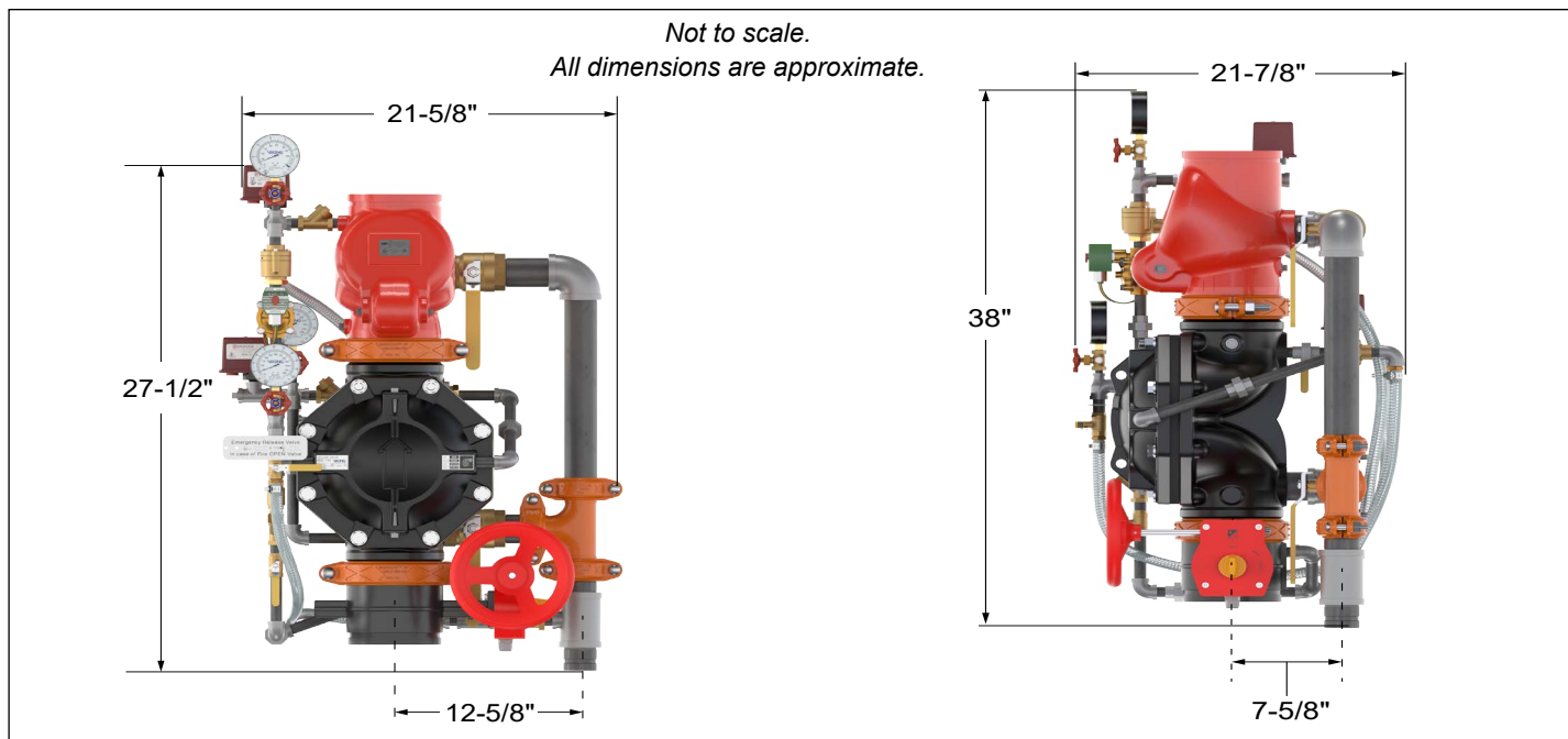
Figure 18: Dimensions - 6" Pre-trimmed Riser
