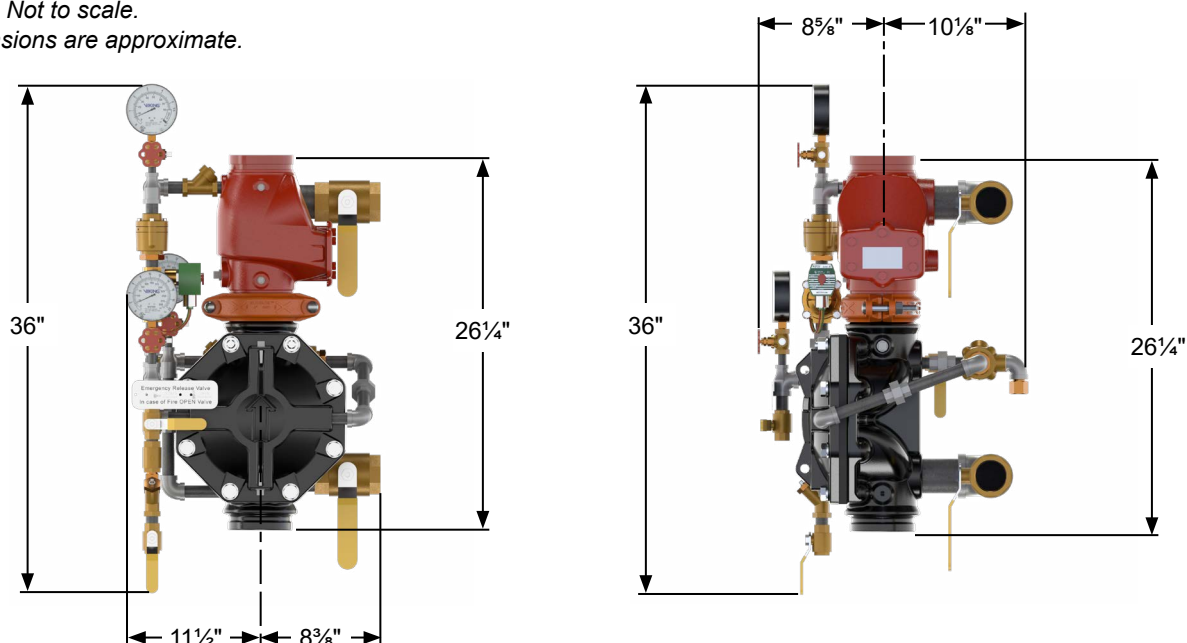
Figure 17: Dimensions - 4" LoosePre-trimmed
