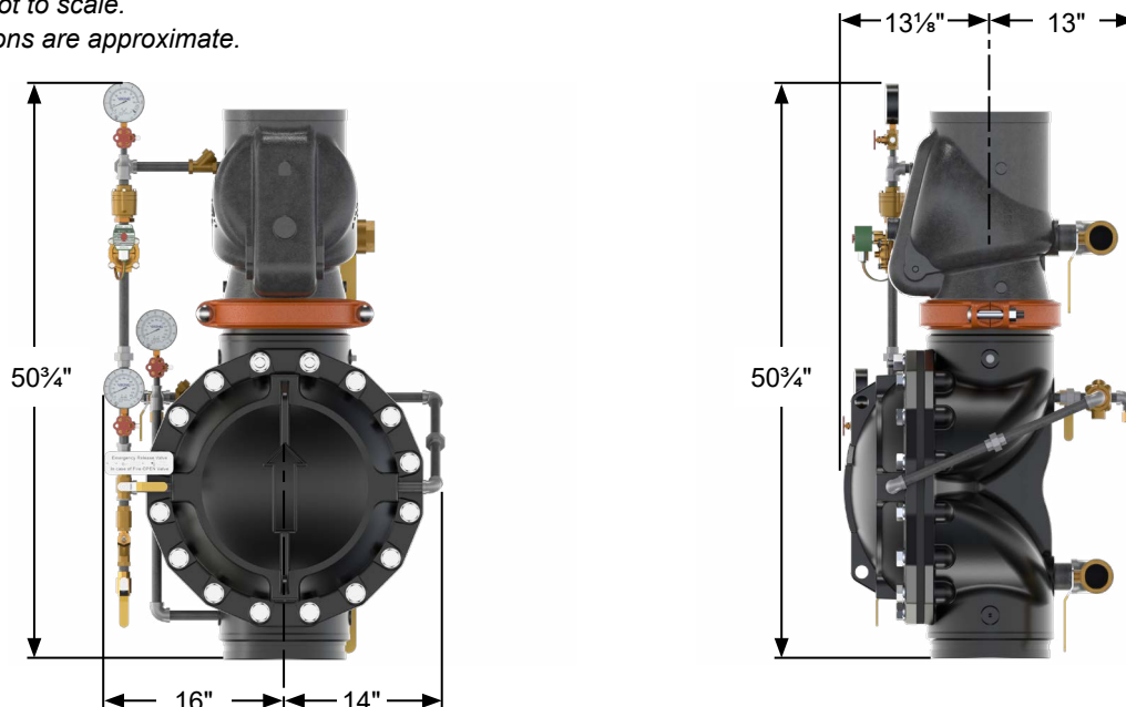
Figure 22: Dimensions - 10" Loose/Pre-trimmed
