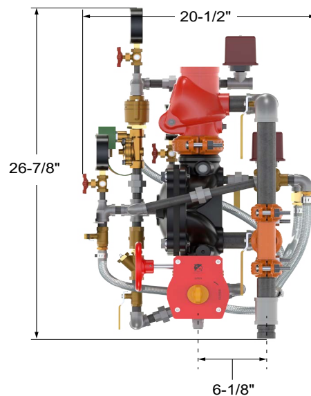
Figure 14: Dimensions - 3" Pre-trimmed Riser
