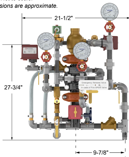
Figure 8: Dimensions - 1-1/2" Pre-trimmed Riser
