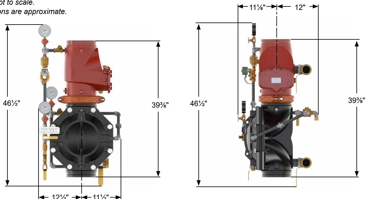
Figure 21: Dimensions - 8" Loose/Pre-trimmed
