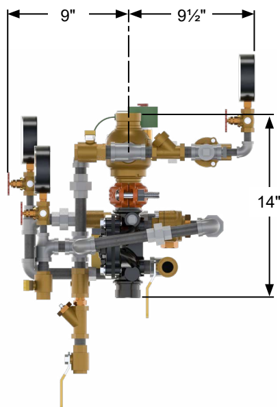
Figure 9: Dimensions - 1-1/2" Loose/Pre-trimmed
