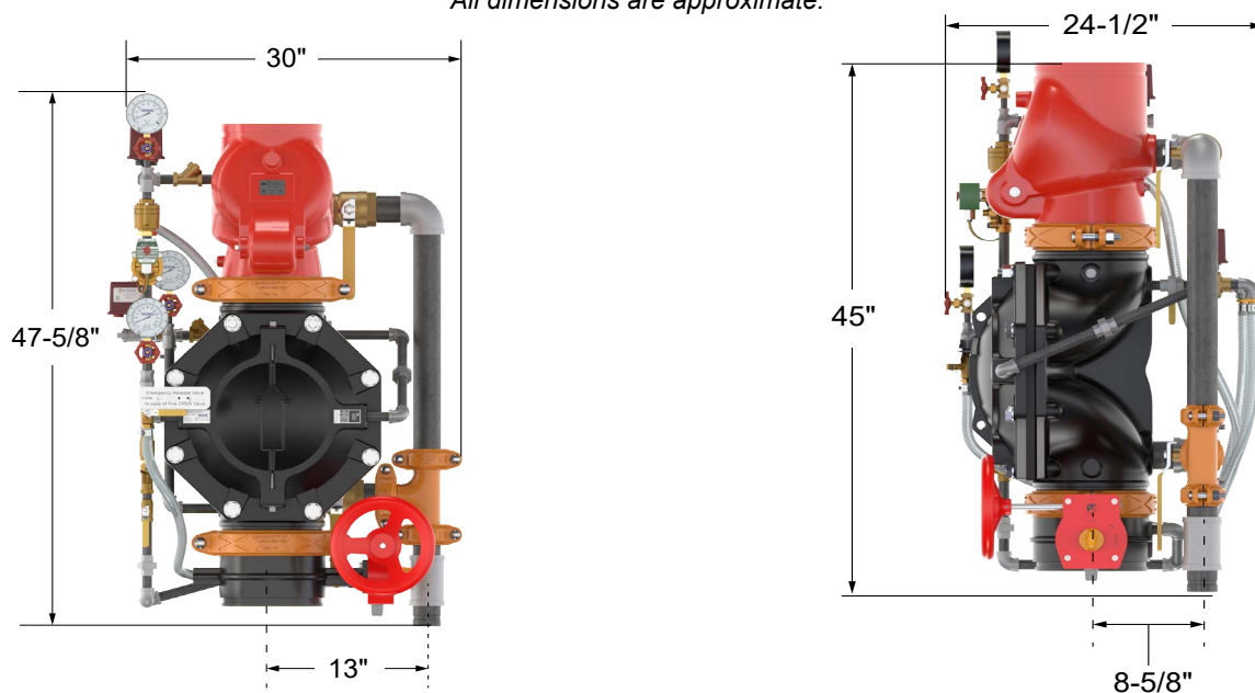
Figure 20: Dimensions - 8" Pre-trimmed Riser
