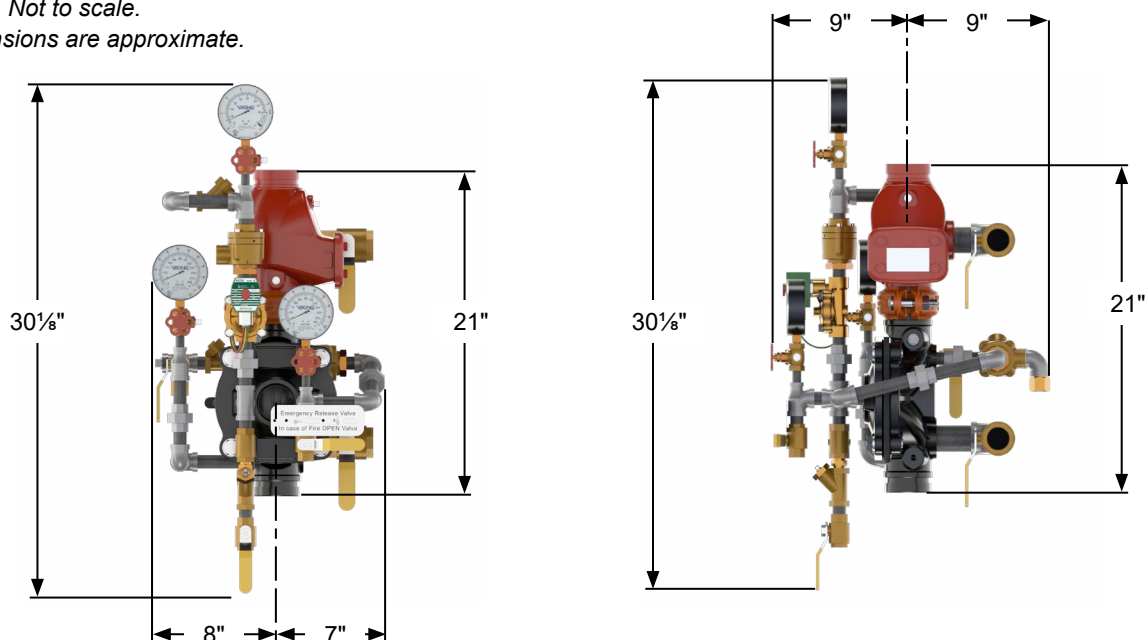
Figure 13: Dimensions - 2 1/2" Loose/Pre-trimmed
