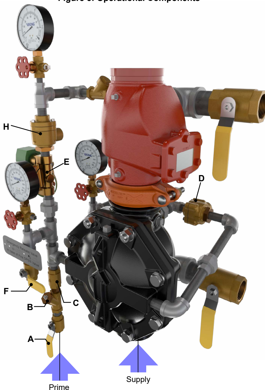
Figure 5: Operational Components
