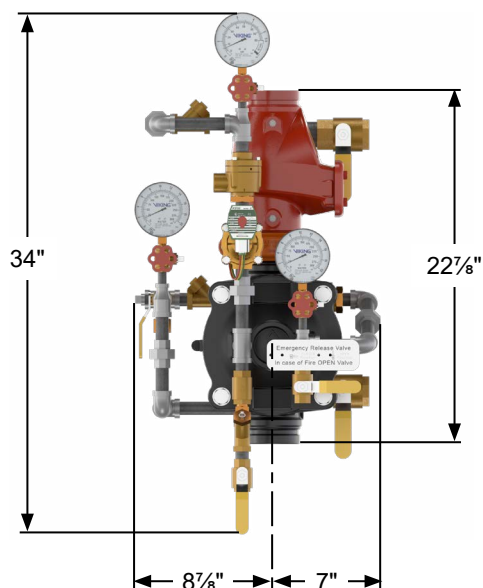
Figure 15: Dimensions - 3" Loose Pre-trimmed
