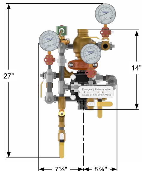
Figure 9: Dimensions - 1-1/2" Loose/Pre-trimmed
