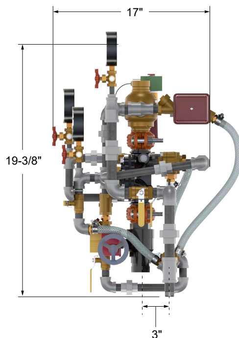
Figure 8: Dimensions - 1-1/2" Pre-trimmed Riser
