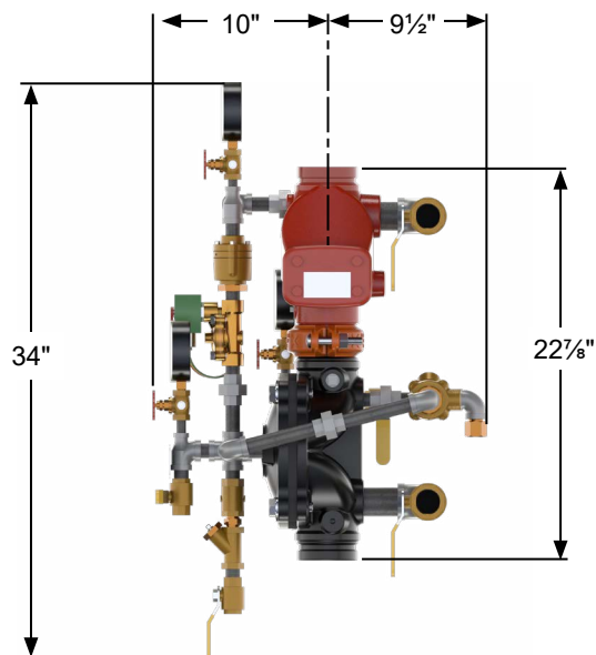
Figure 15: Dimensions - 3" Loose Pre-trimmed
