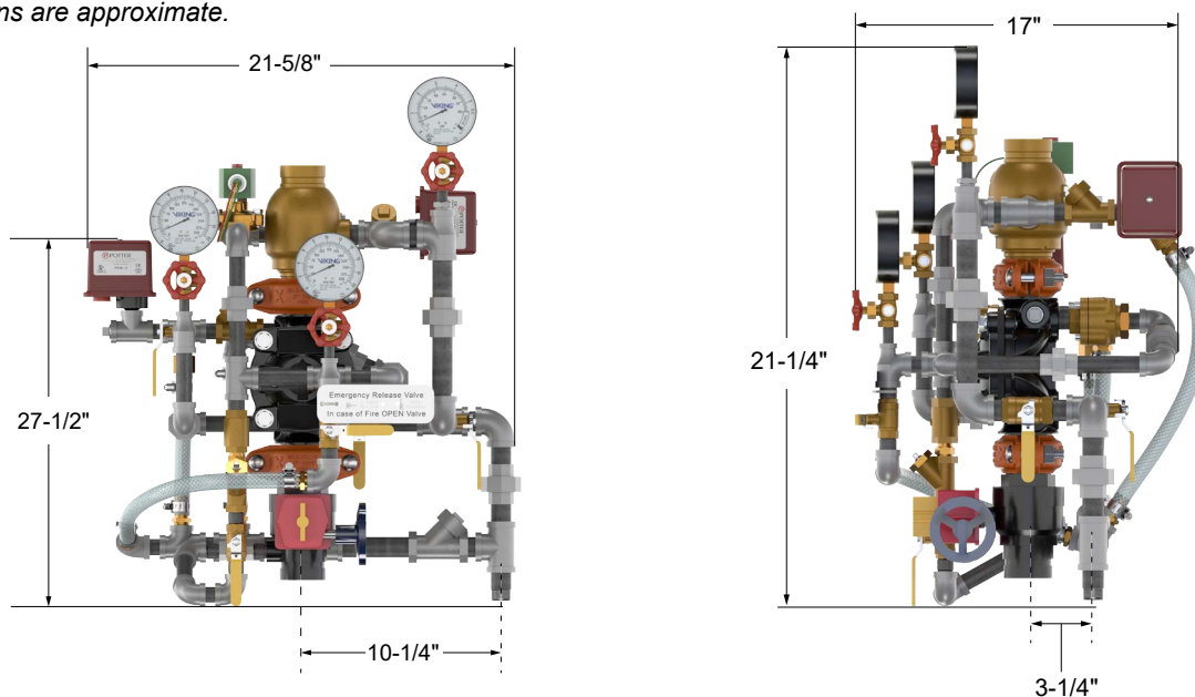
Figure 10: Dimensions - 2" Pre-trimmed Riser
