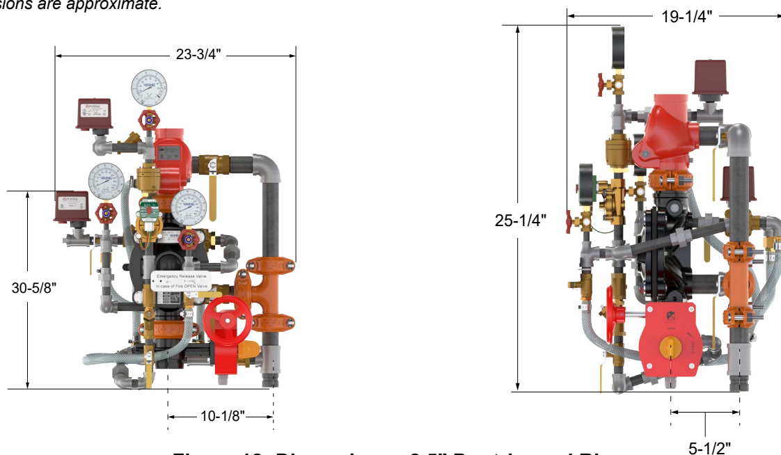
Figure 12: Dimensions - 2.5" Pre-trimmed Riser
