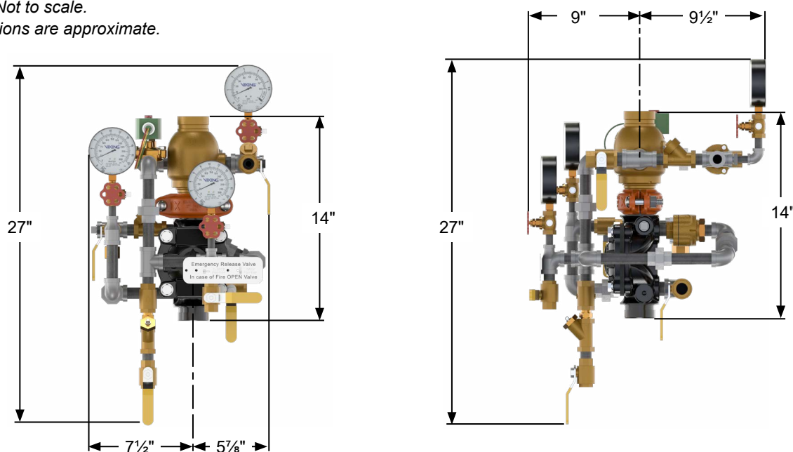
Figure 11: Dimensions - 2" Loose/Pre-trimmed
