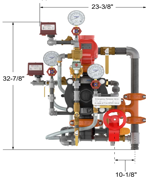
Figure 14: Dimensions - 3" Pre-trimmed Riser
