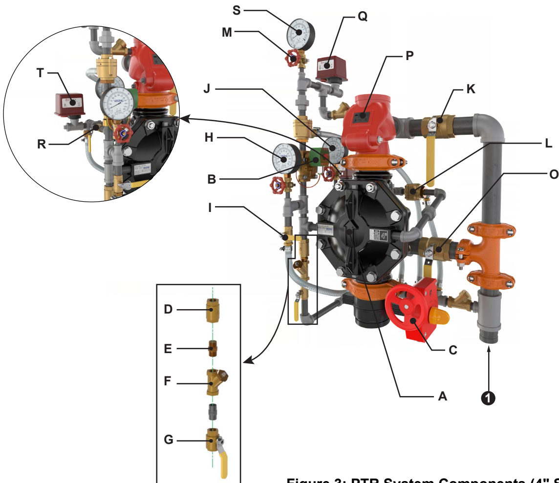
Figure 3: PTR System Components (4" Shown)
