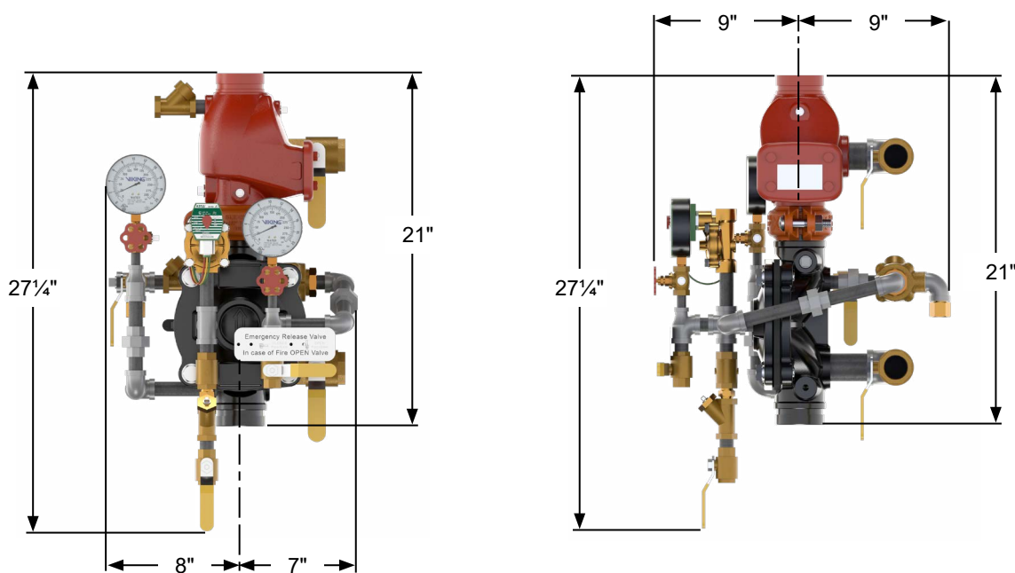
Figure 10: Dimensions - 2 1/2" Pre-Trimmed/Loose
