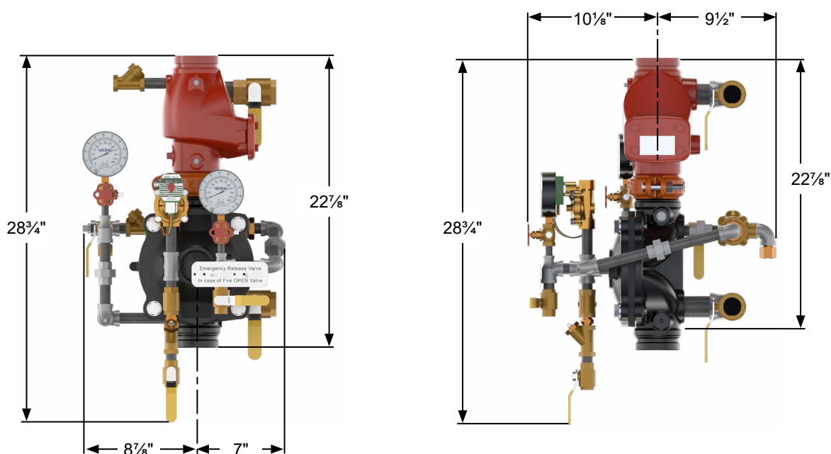
Figure 11: Dimensions - 3" Pre-Trimmed/Loose Not to scale. All dimensions are approximate.
