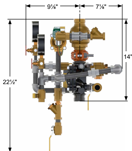
Figure 8: Dimensions - 1-1/2" Pre-Trimmed/Loose
