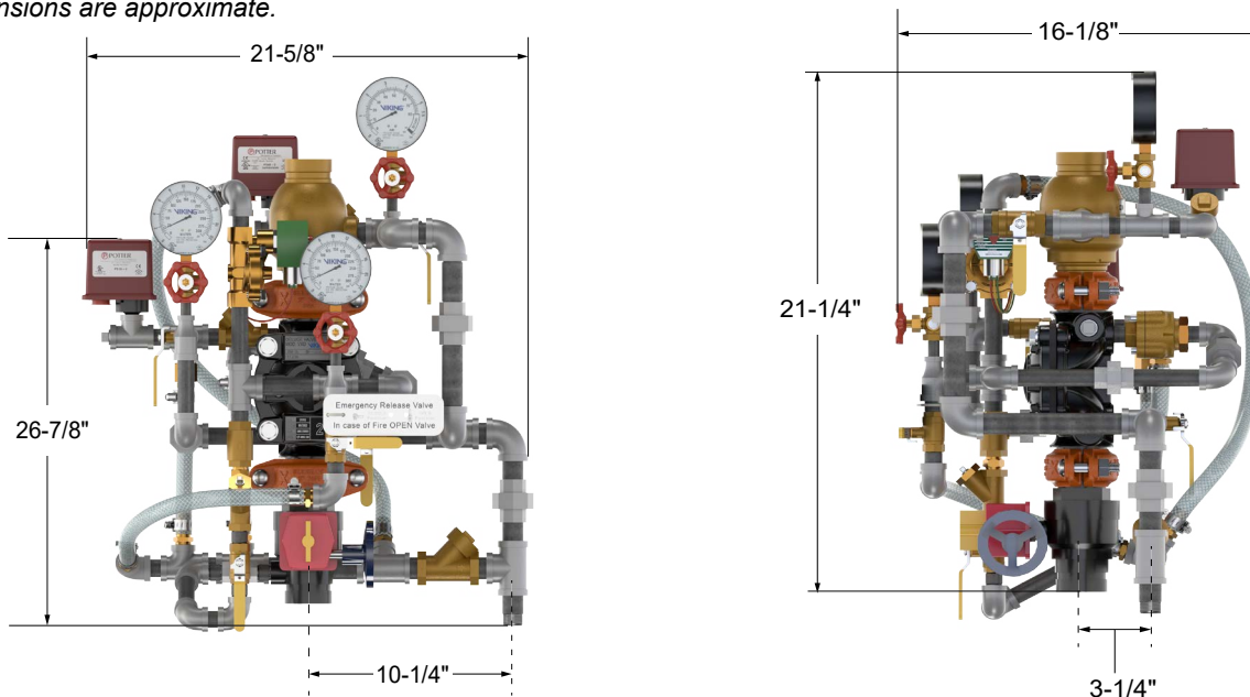
Figure 10: Dimensions - 2" Pre-trimmed Riser
