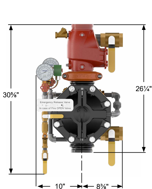
Figure 12: Dimensions - 4"
