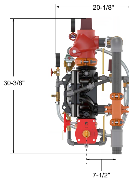
Figure 16: Dimensions - 4" Pre-trimmed Riser
