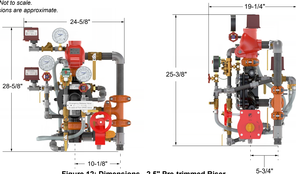
Figure 12: Dimensions - 2.5" Pre-trimmed Riser
