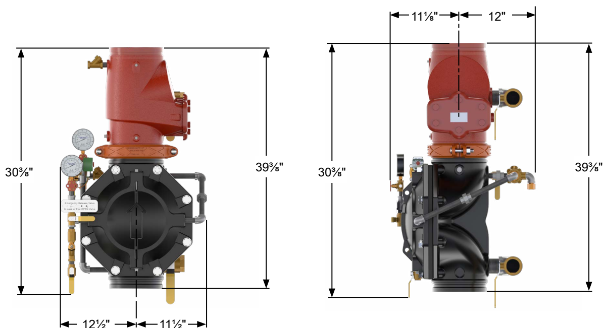
Figure 14: Dimensions - 8"
