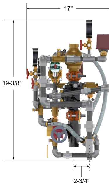
Figure 8: Dimensions - 1-1/2" Pre-trimmed Riser
