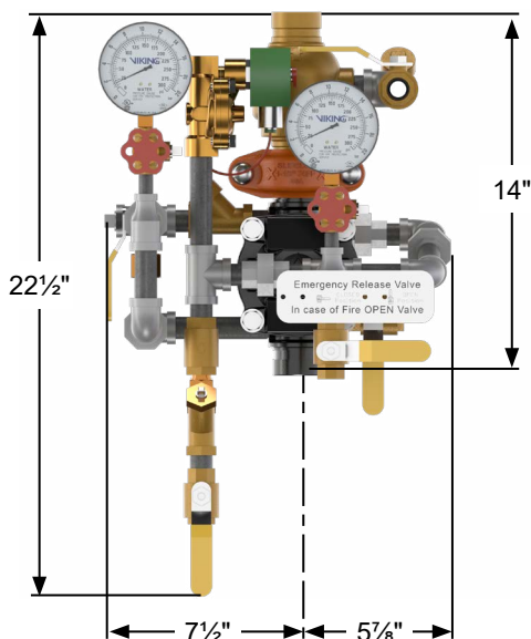
Figure 8: Dimensions - 1-1/2" Pre-Trimmed/Loose
