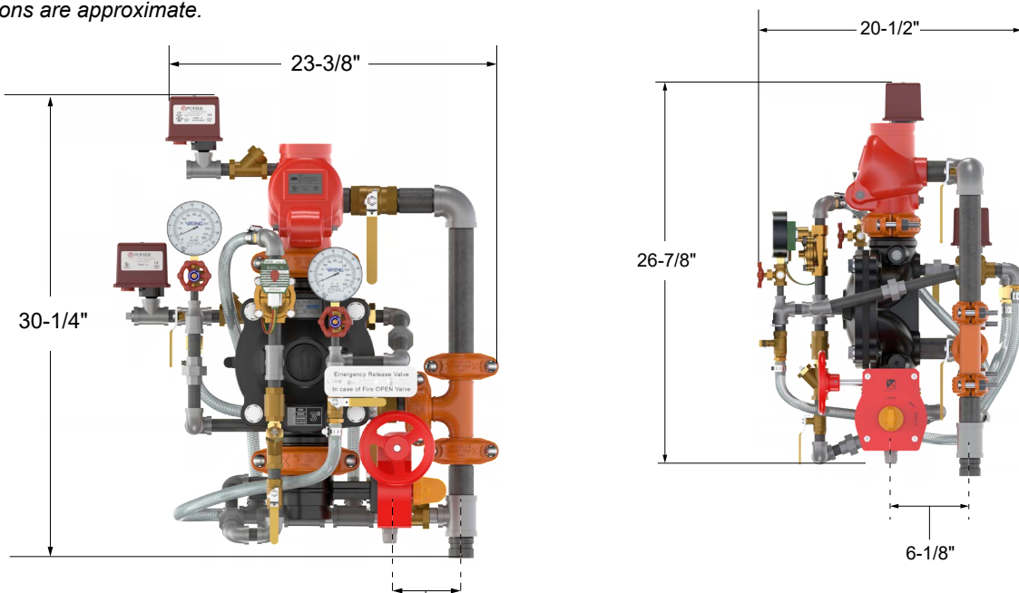
Figure 14: Dimensions - 3" Pre-trimmed Riser
