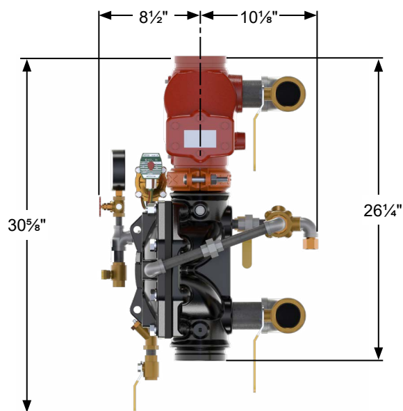
Figure 12: Dimensions - 4"
