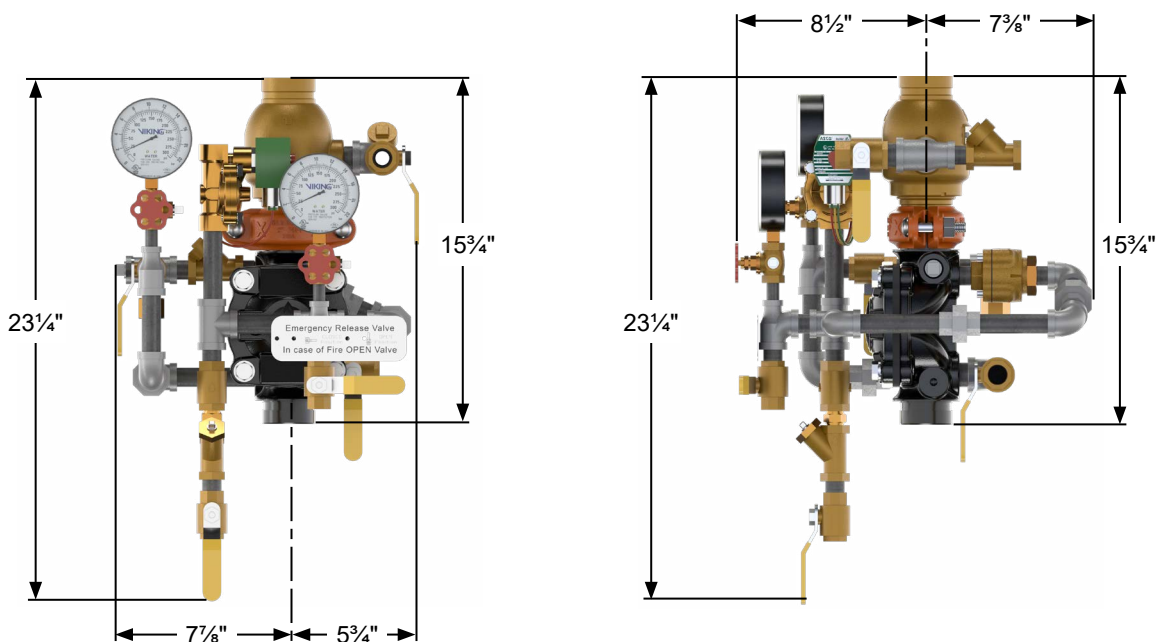
Figure 9: Dimensions - 2" Pre-Trimmed/Loose
