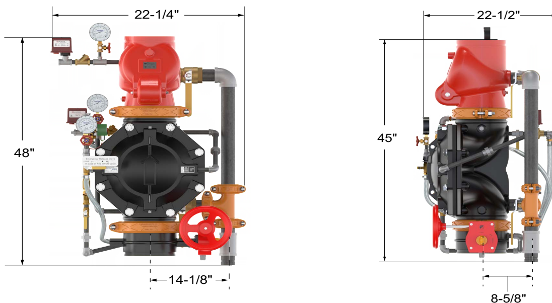
Figure 20: Dimensions - 8" Pre-trimmed Riser
