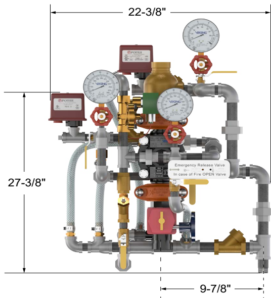
Figure 8: Dimensions - 1-1/2" Pre-trimmed Riser
