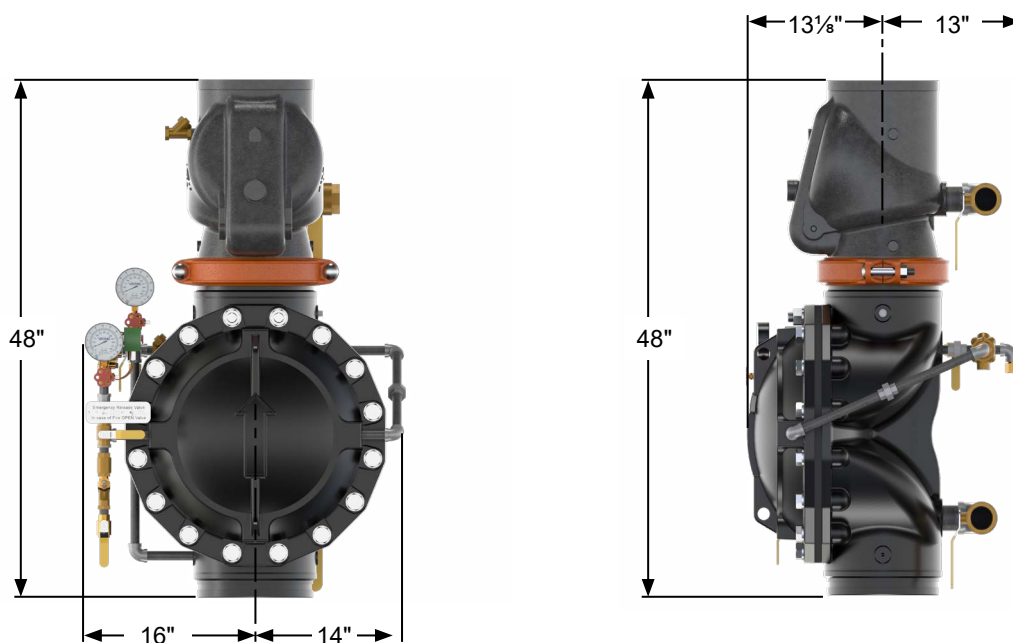
Figure 15: Dimensions - 10"
