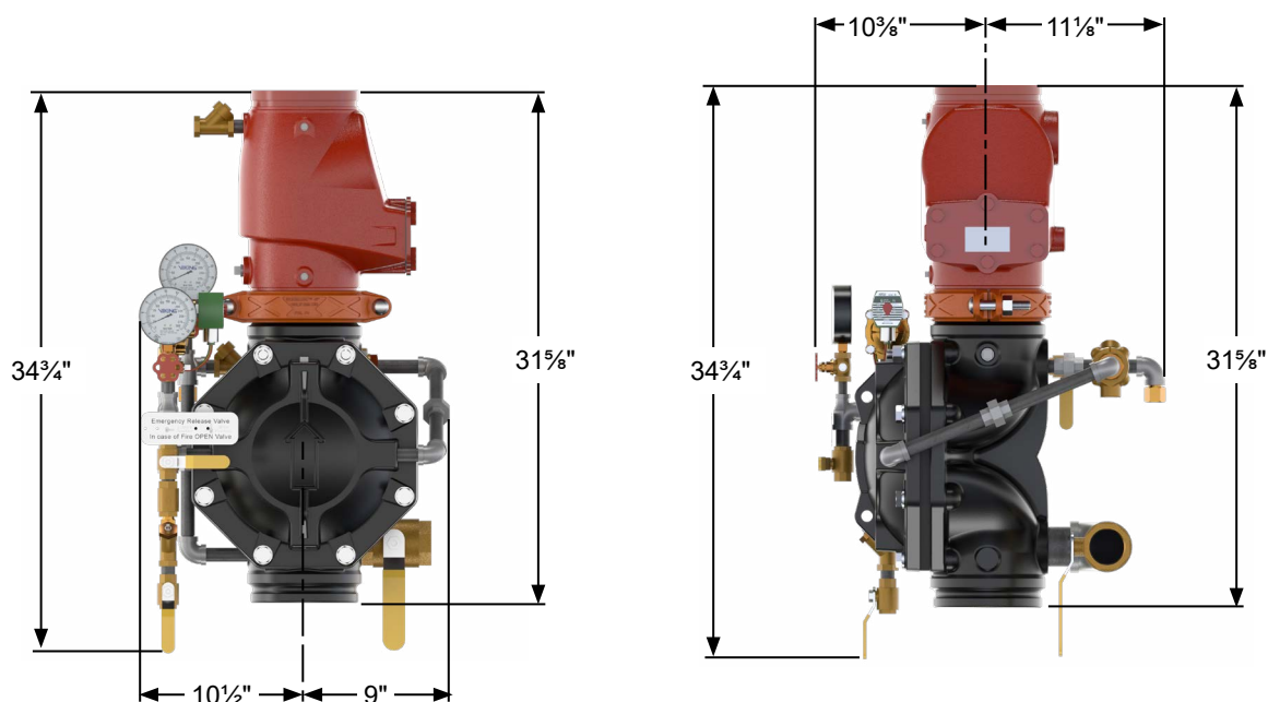
Figure 13: Dimensions - 6"
