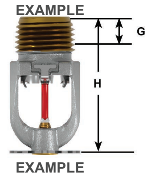
Figure – 2: Dimensions
