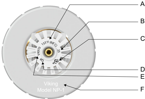
Figure – 1: Markings and Dimensions
