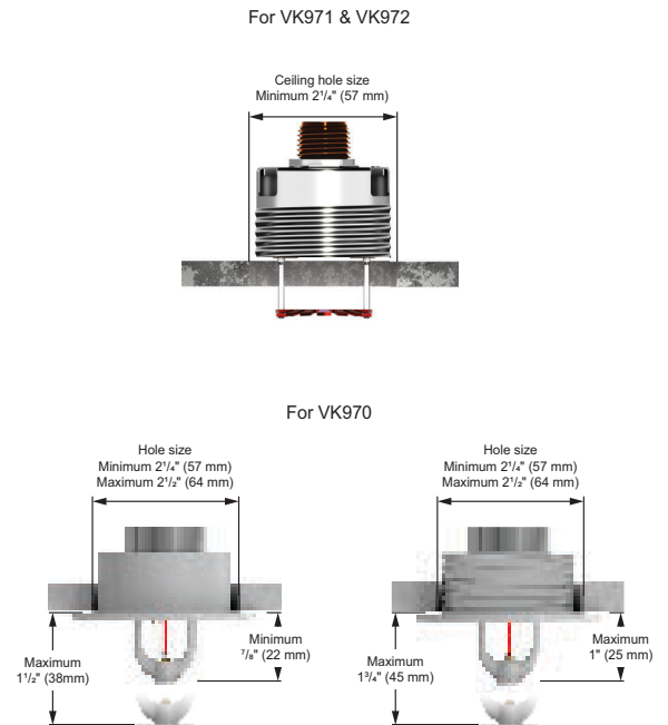
Figure – 1: Installation Clearances and Dimensions
