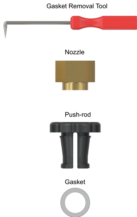
Figure – 1: Repair Kit Components
