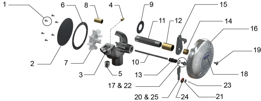
Figure – 4 Water Motor Alarm Components
