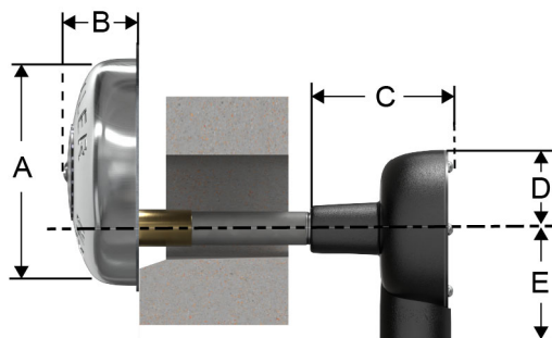
Figure – 1: Water Motor Alarm Dimensions
