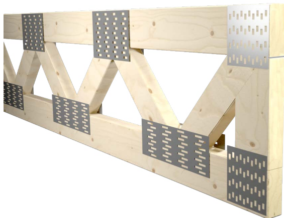
Example of Typical 2x4 Construction Refer to Design Criteria
