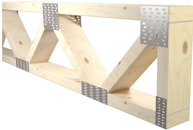
Example of Typical 2x4 Construction Refer to Design Criteria
