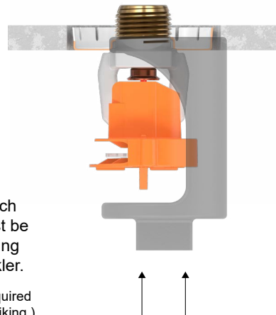
Figure 2: Wrench 13577W/B for Recessed Sprinkler
