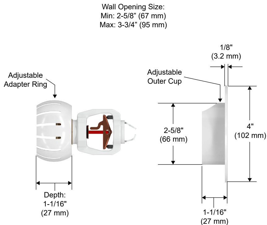
Figure 6: Sprinkler VK486 Dimensions with the Model G-1 Escutcheon
