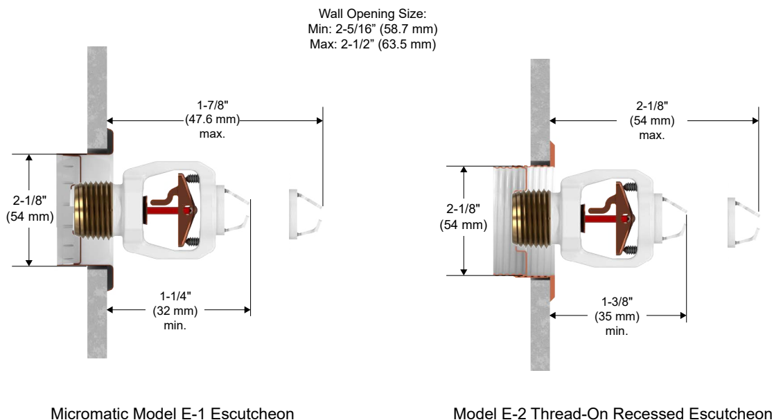
Figure 5: Sprinkler VK486 Dimensions with the Model E-1 and E-2 Recessed Escutcheons
