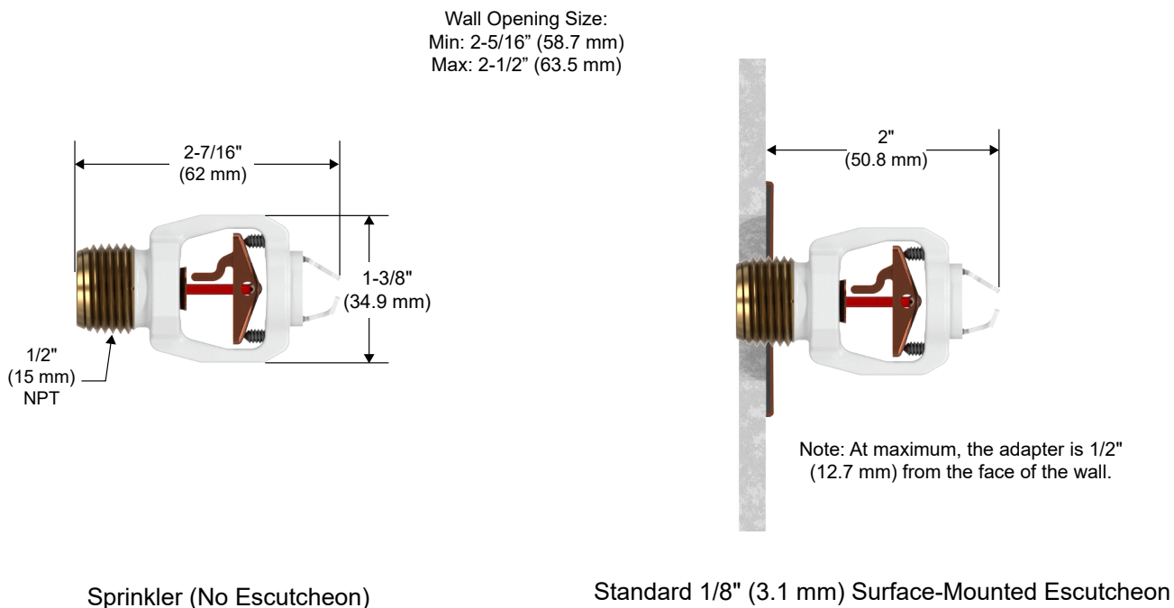
Figure 4: Sprinkler VK486 Dimensions with a Standard Escutcheon
