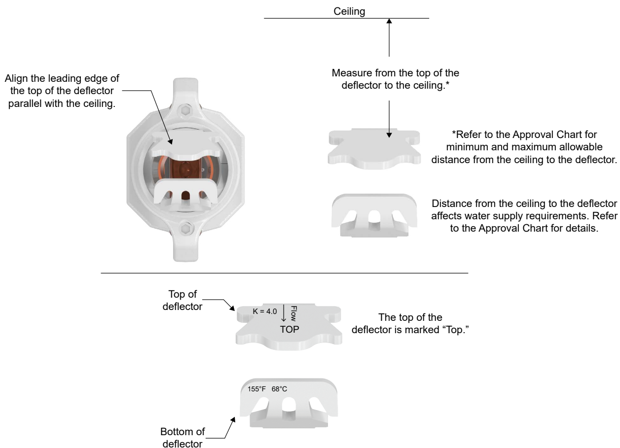
Figure 3: Correct Orientation of the Deflector
