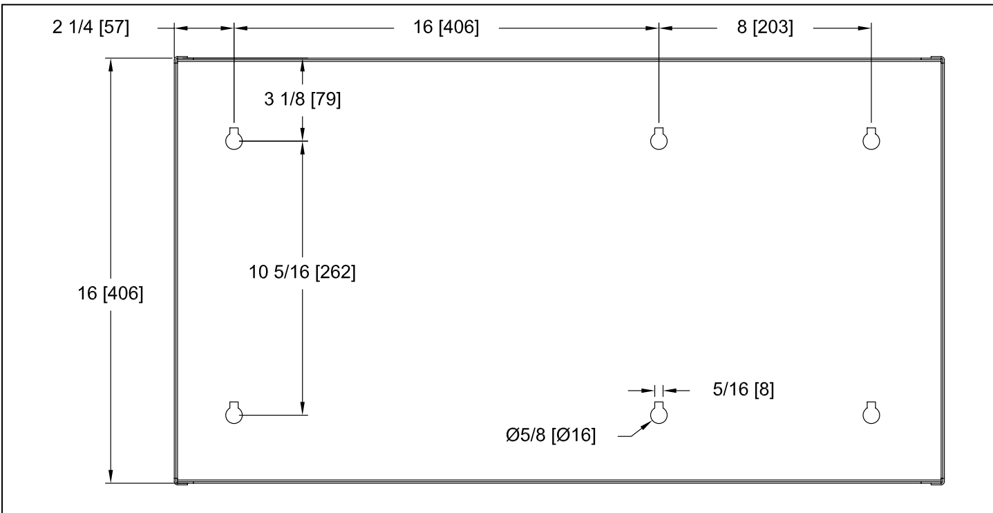
Figure 10 - Trimpac Components (Items B.1 - B.12)
