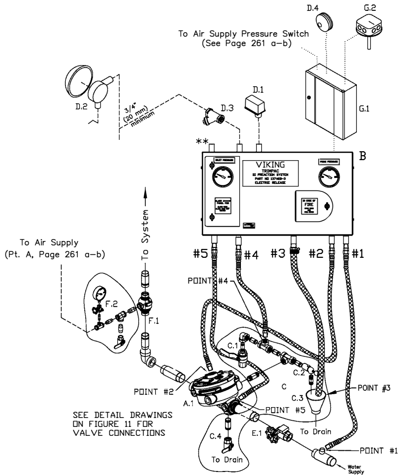
SINGLE INTERLOCKED PREACTION SYSTEM WITH ELECTRIC RELEASE
