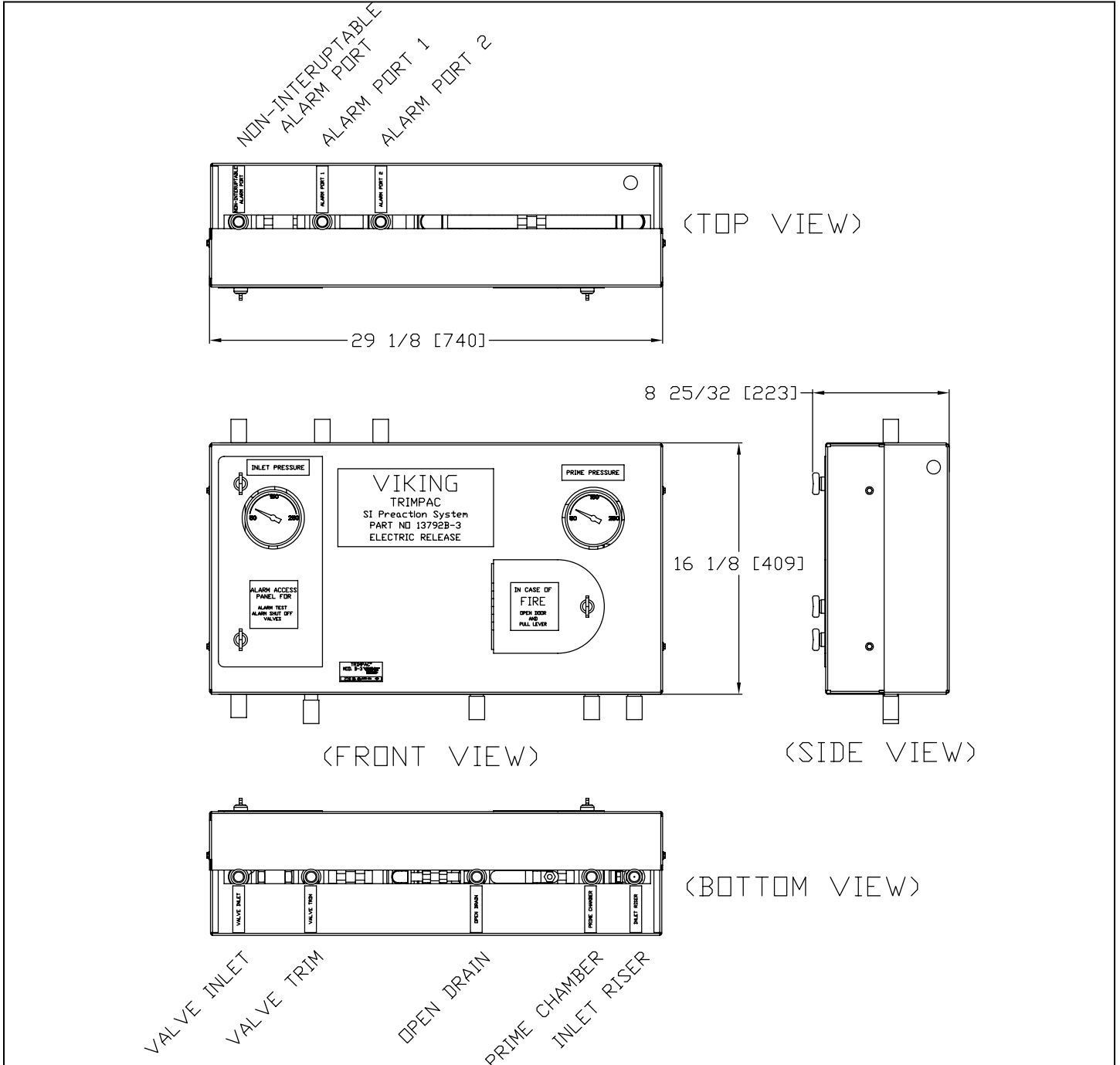
Figure 2 - Trimpac® Model B-3 Dimensions
