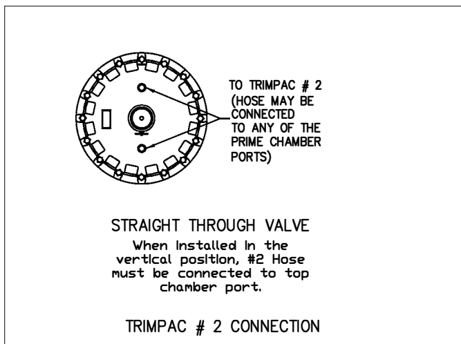
Figure 9 - Valve Connections
