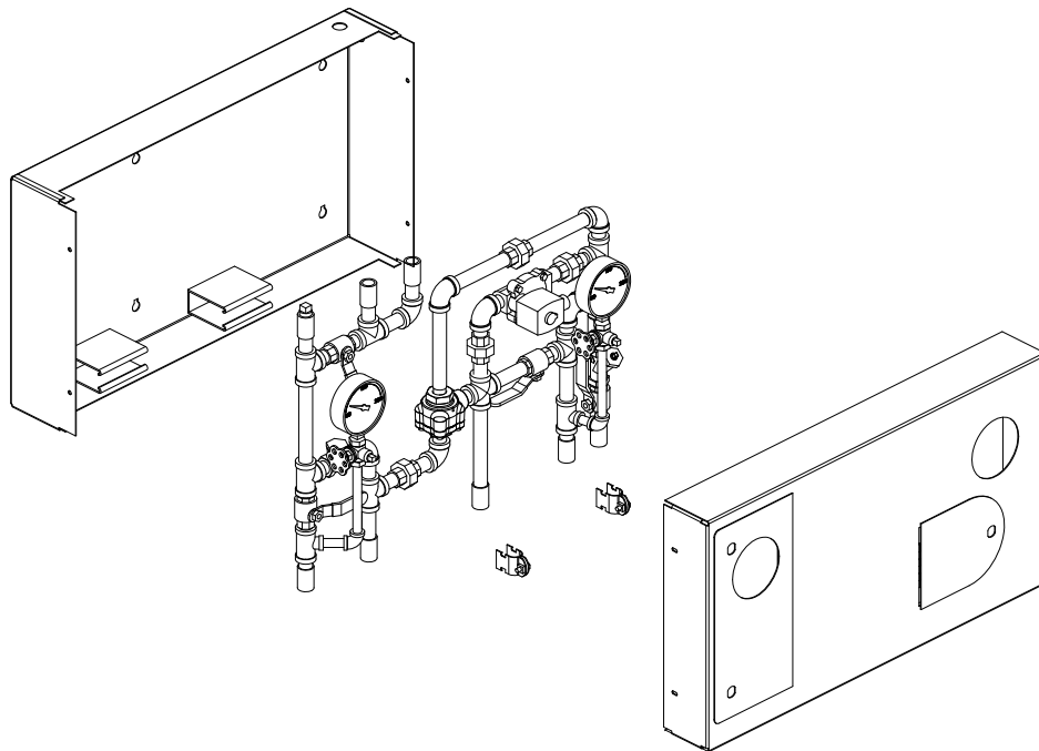
Figure 1 - Isometric View
