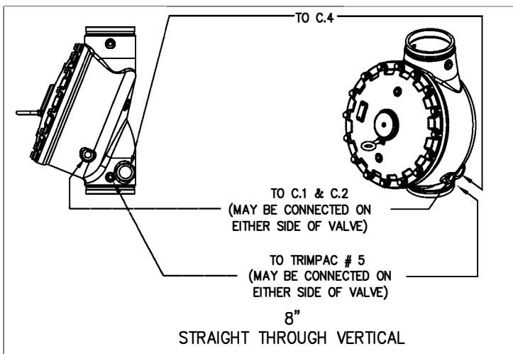
Figure 9 - Valve Connections
