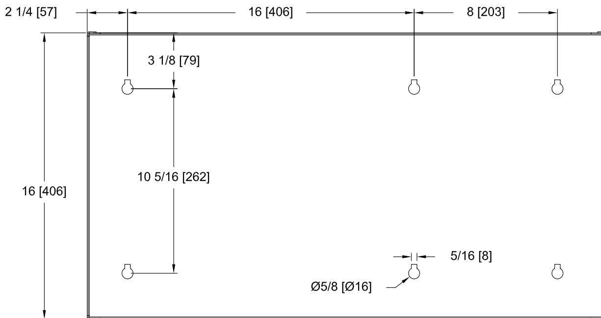
Figure 11 - Mounting Dimensions
