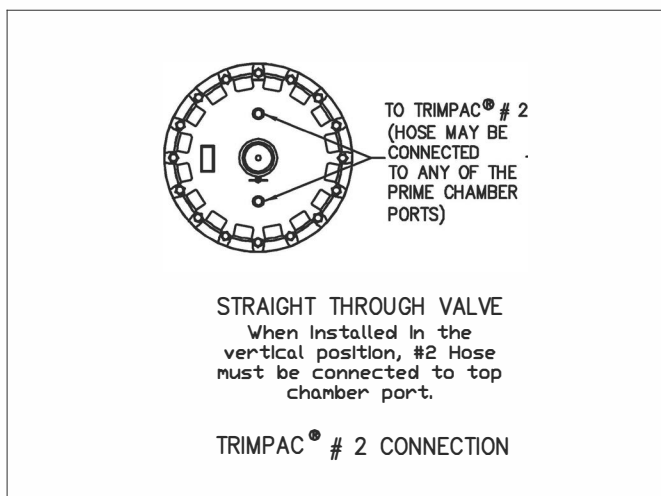
Figure 9 - Valve Connections
