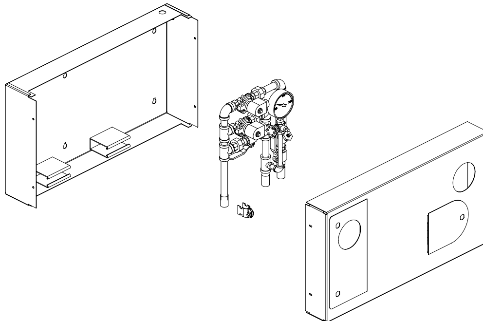
Figure 1 - Isometric View
