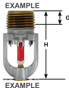
Figure – 2: Dimensions
