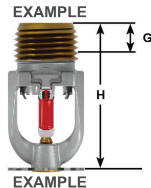
Figure – 2: Dimensions
