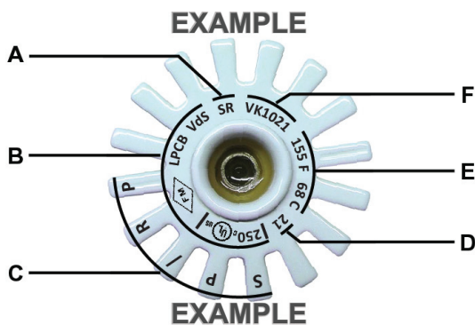
Figure – 1: Markings
