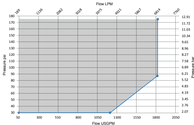
6" CAVITATION CHART
