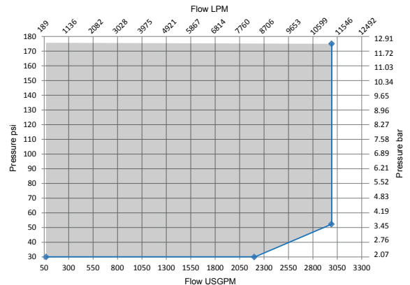
8" CAVITATION CHART
